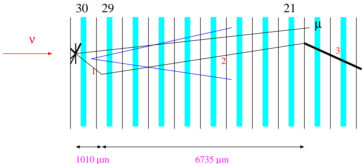
Figure 2: Sketch of the event topology in emulsion. Emulsion plates are indicated by two vertical white bars (the sensitive emulsion layers) around a shaded vertical bar (the plastic base). A discussion of the tracks can be found in the text.
