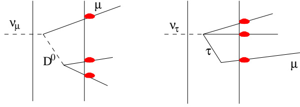
Figure 1: Topology of \nu_\mu interactions with D^0 production and subsequent in-plate D^0 decay (left) compared to \nu_\tau interactions with subsequent in-plate tau decay (right). The shaded regions on the tracks indicate the 100\ \mu\text{m} layer where tracks are automatically searched for in emulsion.
