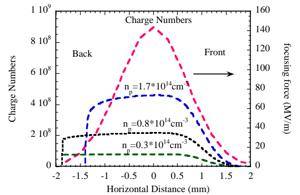
Figure 1: Beam charge distribution and the transverse focusing force witnessed by the beam electrons \sigma_r away from the axis of ion channel from Particle-in-Cell simulation (Quasi-Static Appr.) at 3 different plasma densities.
