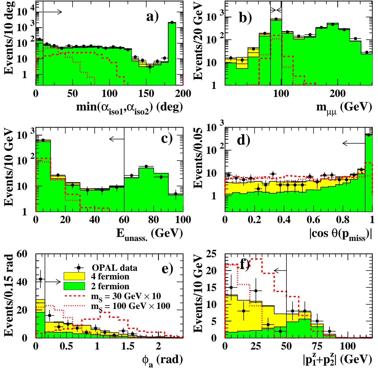
Figure 6: Cut variables for Z^0 \rightarrow \mu^+\mu^- at \sqrt{s} = 183\text{-}209\text{ GeV} . The OPAL data are indicated by dots with error bars (statistical error), the four-fermion background by the light grey histograms and the two-fermion background by the medium grey histograms. The signal distributions from a 30\text{ GeV } S^0 are plotted as dashed lines and those from a 100\text{ GeV } S^0 as dotted lines, respectively. The signal histograms are normalised to 10 and 100 times of the Standard Model Higgs-strahlung cross section, respectively, and show the decays S^0 \rightarrow gg . Each variable is shown with the cuts applied before the cut on this variable is done, respecting the order of cuts in Table 4. The arrows indicate the accepted regions.
