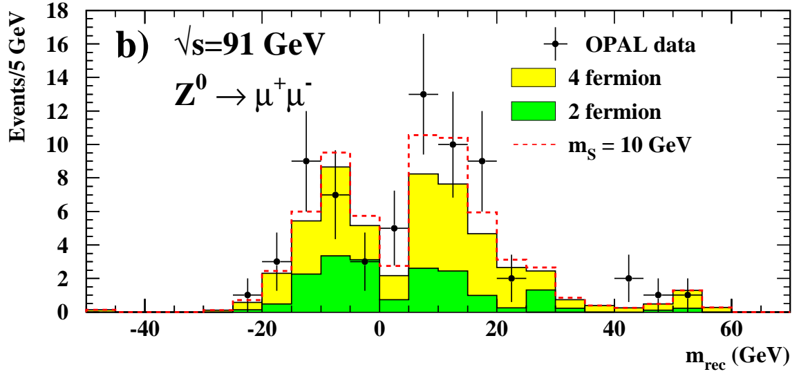
Figure 4: The recoil mass spectra from \sqrt{s} = 91.2 \text{ GeV} a) for the decays Z^0 \rightarrow e^+e^- and b) for Z^0 \rightarrow \mu^+\mu^- . OPAL data are indicated by dots with error bars (statistical error), the four-fermion background by the light grey histograms and the two-fermion background by the dark grey histograms. The dashed lines for the signal distributions are plotted on top of the background distributions with normalisation corresponding to the cross section excluded at 95% confidence level from the combination of both channels.
