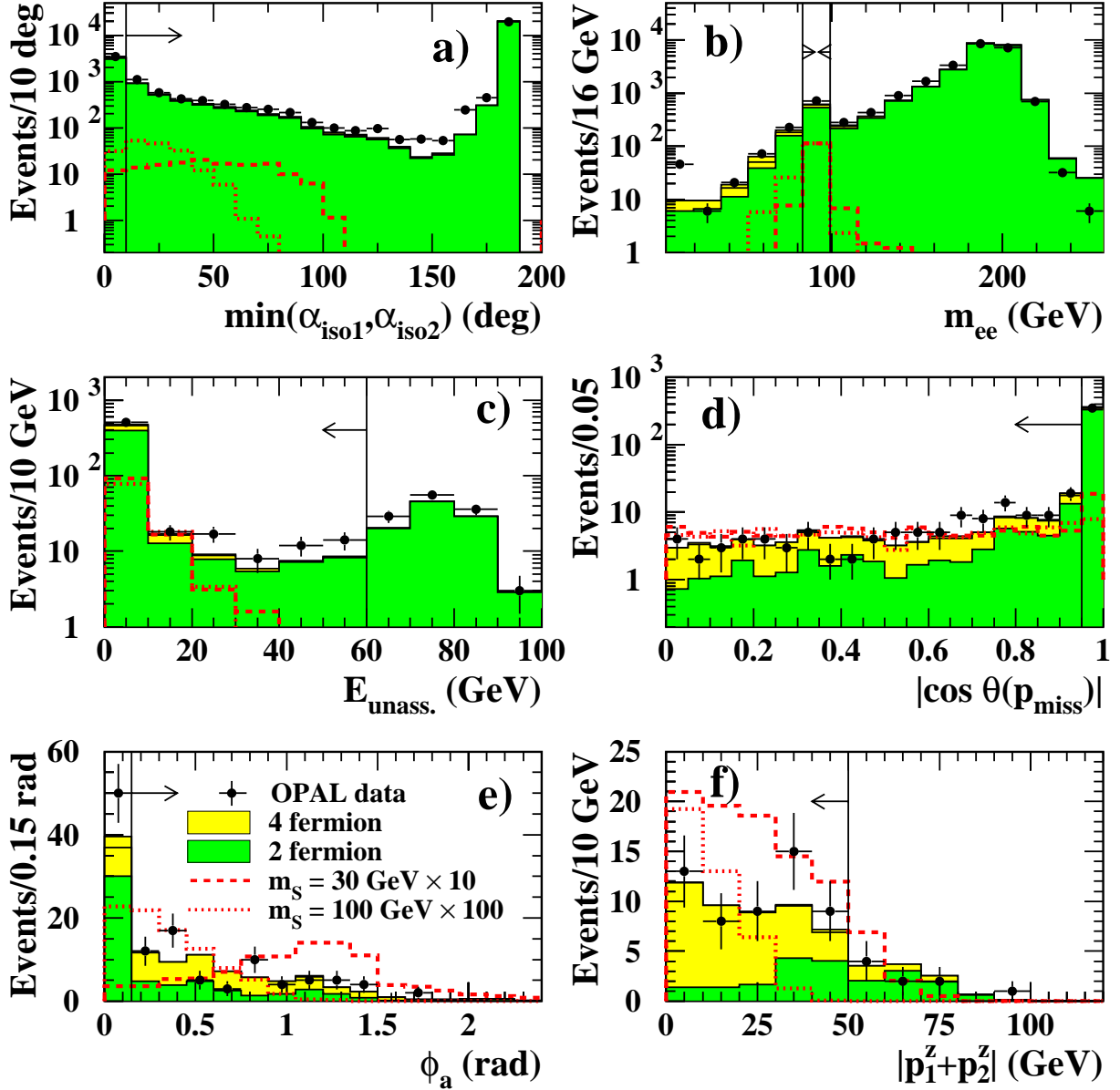
Figure 5: Cut variables for Z^0 \rightarrow e^+e^- at \sqrt{s} = 183\text{-}209 GeV. The OPAL data are indicated by dots with error bars (statistical error), the four-fermion background by the light grey histograms and the two-fermion background by the medium grey histograms. The signal distributions from a 30 GeV S^0 are plotted as dashed lines and those from a 100 GeV S^0 as dotted lines, respectively. The signal histograms are normalised to 10 and 100 times of the Standard Model Higgs-strahlung cross section, respectively, and show the decays S^0 \rightarrow gg . Each variable is shown with the cuts applied before the cut on this variable is done, respecting the order of cuts in Table 4. The arrows indicate the accepted regions.
