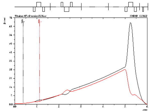
Figure 6. Last 6 m of the beam transport line.
