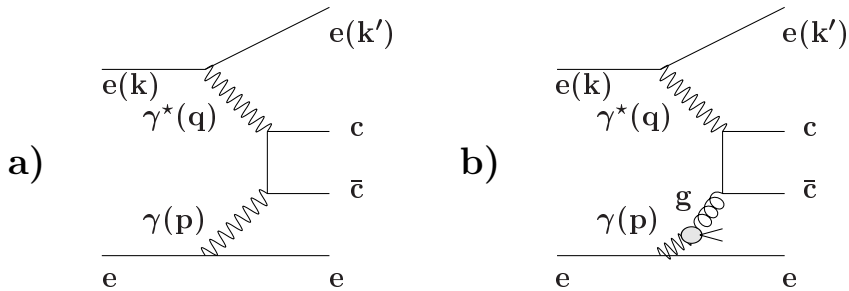
Figure 1: Examples of leading order diagrams contributing to a) the point-like, and b) the hadron-like part of F_{2,c}^{\gamma} .
