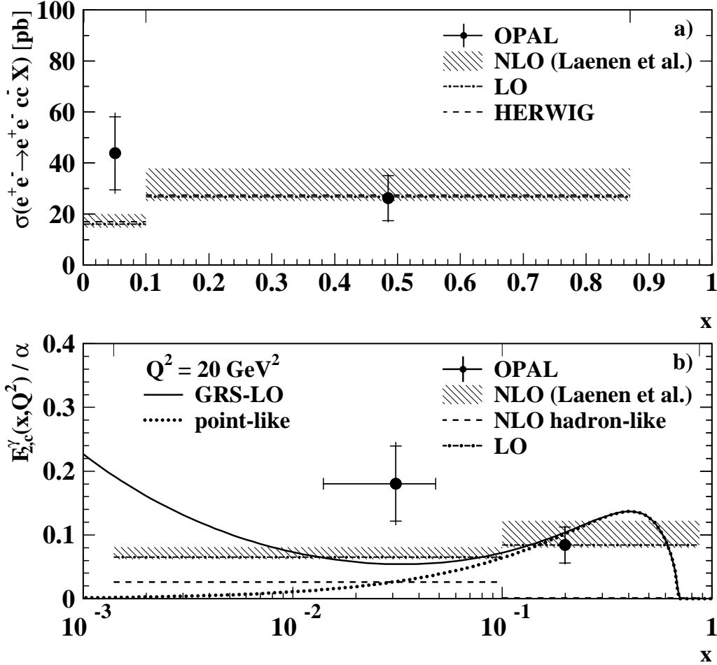
Figure 4: OPAL results for a) the cross-section \sigma(e^+e^- \rightarrow e^+e^- c\bar{c}X) , with 5 < Q^2 < 100 \text{ GeV}^2 and b) for the charm structure function of the photon divided by the fine structure constant, F_{2,c}^\gamma(x, Q^2)/\alpha , at Q^2 = 20 \text{ GeV}^2 . The data points are the results obtained with the HERWIG Monte Carlo model. The outer error bar is the total error and the inner error bar the statistical error. The data points in b) are placed at those x values that correspond to the average predicted F_{2,c}^\gamma within a bin. The data are compared to the calculation of [2] performed in LO and NLO. The band for the NLO calculation indicates the theoretical error from uncertainties in the charm quark mass and renormalisation and factorisation scales. In a) the cross-section prediction of the HERWIG Monte Carlo model is also given. b) also shows the prediction of the GRS-LO parametrisation for the structure function at Q^2 = 20 \text{ GeV}^2 and its point-like component separately.
