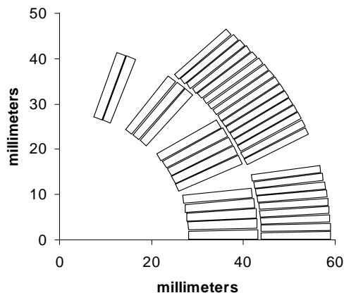
Fig. 3. The upper right quarter of the dipole winding. Together with other quarters it creates the irregular and bent stacks.
