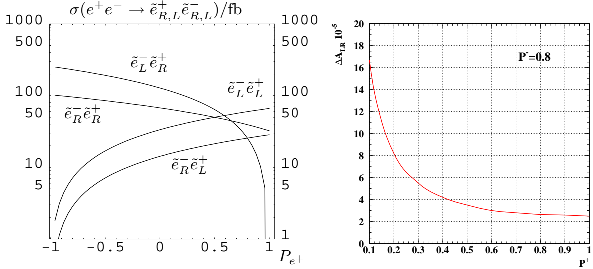
FIG. 9: Two examples of the advantages of e^- and e^+ polarisation in studying new physics and performing precision tests of the SM. Left: cross section for the production of the supersymmetric electron partners as a function of the positron beam polarisation \mathcal{P}_{e^+} (from [44]). Right: statistical uncertainties for left-right asymmetry A_{LR} in the e^+e^- \rightarrow Z^0 \rightarrow \ell^+\ell^- reaction, measured operating the LC at the Z^0 pole energy, as a function of the positron beam polarisation (from [7]).
