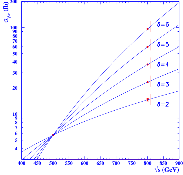
FIG. 11: Determination of the number of extra dimensions from anomalies in the single photon cross section measured at \sqrt{s}=500 GeV and 800 GeV. Points with error bars indicate the expected measurement performed on 500 \text{ fb}^{-1} of data with polarized electron and positron beams. The curves show the expected dependence of the cross section on the collision energy for different number of extra dimensions (from [9]).
