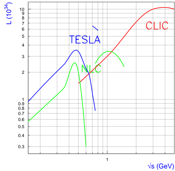
FIG. 13: Estimated luminosity as a function of the \sqrt{s} energy for different LC projects. The two sets of curves for NLC and TESLA refer to the baseline projects where the luminosity is traded for the beam energy, keeping the beam power constant, and to a possible linac upgrade.
