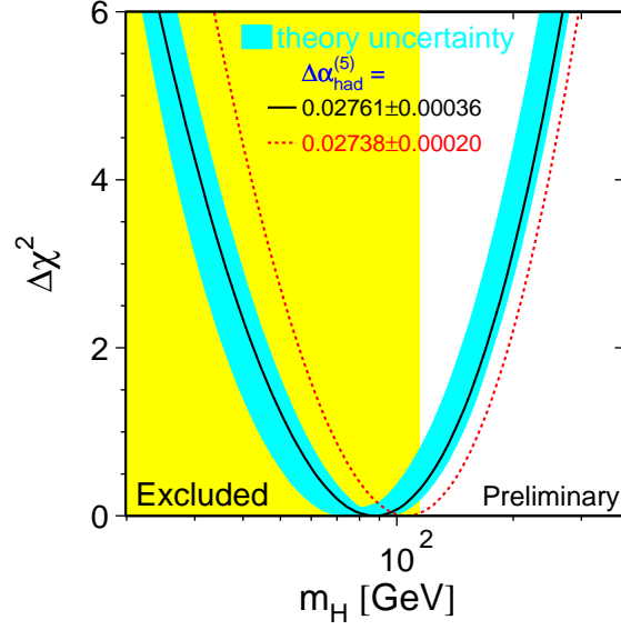
FIG. 1: The \chi^2 of the fit to the electro-weak observables measured at LEP, SLC and Tevatron as a function of the Higgs boson mass. The preferred value is M_H = 88_{-35}^{+53} GeV and the one-sided 95% C.L. upper limit is 196 GeV (from [1])
