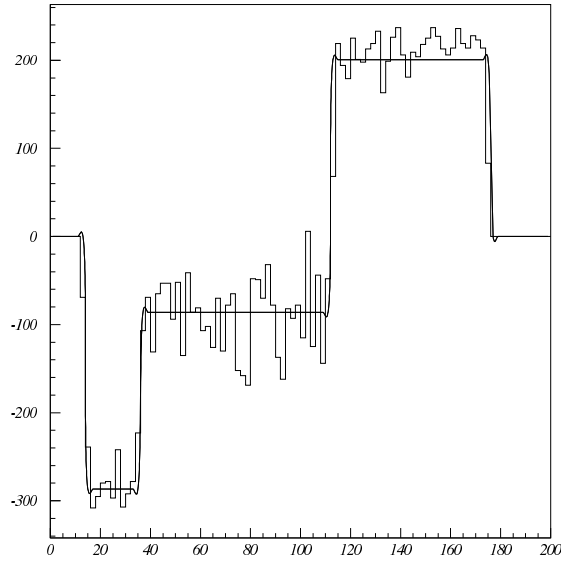
FIG. 6: Example of determinations of masses of sleptons from the measured momentum distribution of muons detected in events produced with different beam polarization states (from [37]).
