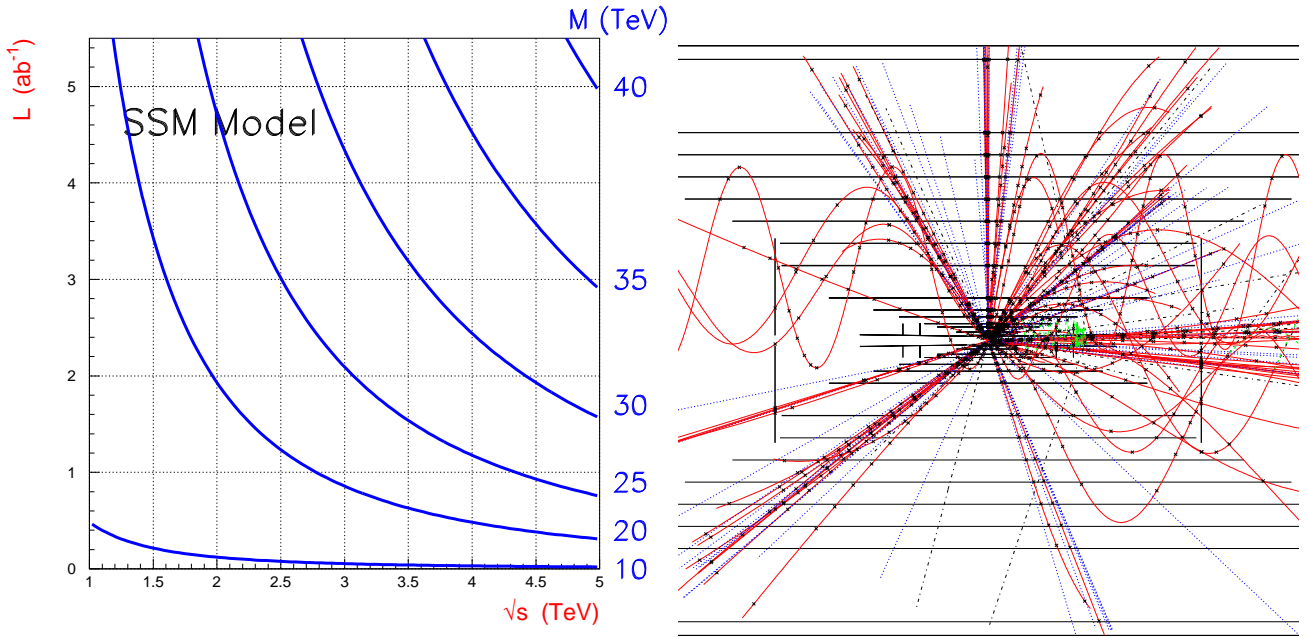
FIG. 12: Examples of multi-TeV physics. Left: the sensitivity to an additional Z' gauge boson through measurements of electro-weak observables as a function the integrated luminosity and center-of-mass energy (from [50]). Right: an event of production and evaporation of a black-hole in 5 TeV e^+e^- collisions (from [5]).
