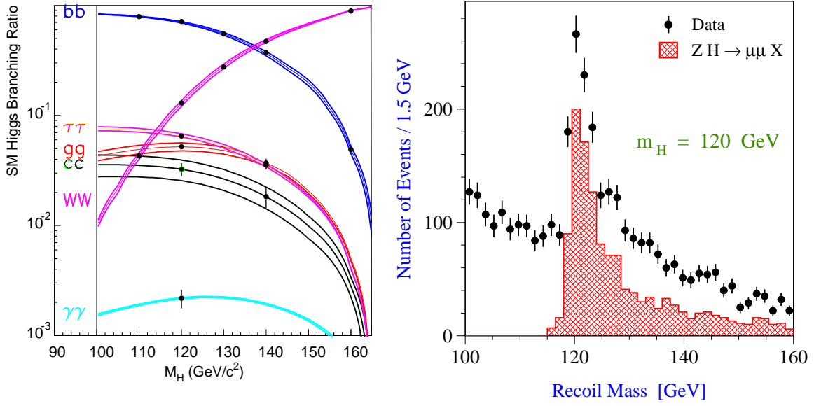
FIG. 5: Left: Higgs decay branching fractions predicted in SM as a function of the Higgs boson mass. The lines represent the expected range due to uncertainties in the input parameters and the points with error bars represent the estimated statistical accuracies obtainable at a LC with 500 \text{ fb}^{-1} (from [30]). Right: reconstructed recoil mass spectrum showing the mass peak due to a 120 GeV Higgs boson produced in the e^+e^- \rightarrow ZH process (from [9]).
