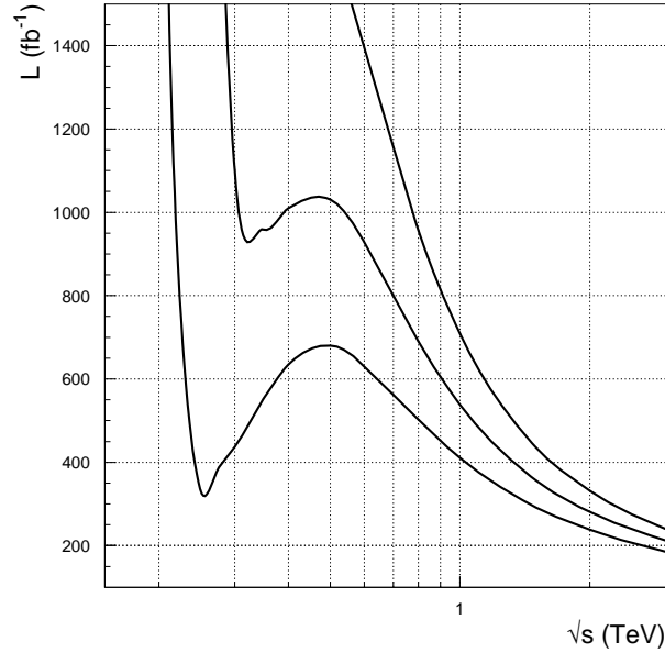
FIG. 2: The scaling of the integrated luminosity, necessary to produce 10^5 Higgs bosons in e^+e^- collisions, with the center-of-mass energy \sqrt{s} for three values of the Higgs mass: 120 GeV, 180 GeV and 240 GeV.
