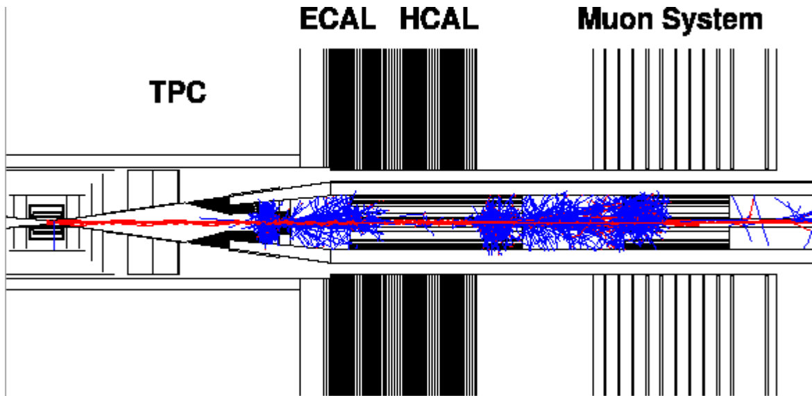
FIG. 3: The LC interaction region with the e^+e^- pair background confined by the solenoidal magnetic field and shielded by a system of forward masks.
