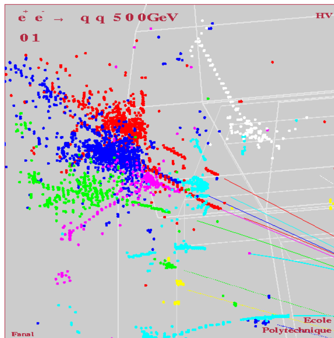
FIG. 8: The response of a tungsten digital hadronic calorimeter to Particles from an hadronic jet (from [38]).
