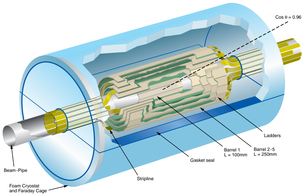
FIG. 4: Isometric view of the Vertex Detector surrounding the interaction region. The concentric layers of high resolution Si pixel detectors ensure the discrimination of charged particles produced in the decay of short-lived heavy hadrons from those originating at the point of beam interaction (from [9]).
