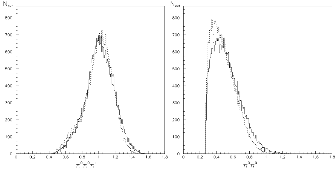
Figure 2: The \bar{\nu}_\tau \pi^0 \pi^0 \pi^0 \pi^+ channel. The left-hand side plots the \pi^0 \pi^0 \pi^0 \pi^+ invariant mass distribution and the right-hand side is the \pi^0 \pi^0 invariant mass distribution. The continuous and dotted lines correspond to the old CLEO and new Novosibirsk current respectively.
