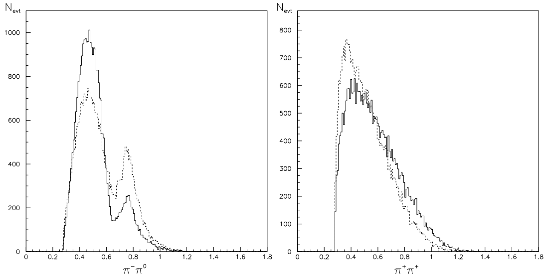
Figure 6: The \bar{\nu}_\tau \pi^+ \pi^+ \pi^- \pi^0 channel. The left-hand side plots the \pi^- \pi^0 invariant mass distribution and the right-hand side is the \pi^+ \pi^+ invariant mass distribution. The continuous and dotted lines correspond to the old CLEO and new Novosibirsk current respectively.
