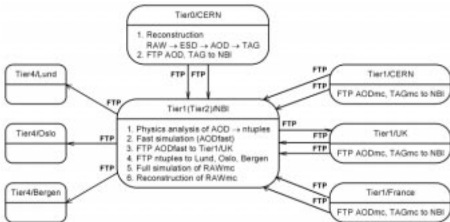
Figure 1: The example used in the simulation. If NBI is a Tier2, it is assumed that the full simulation results (AOD, TAG) are transferred to the centre from three Tier1 centres (in France, at CERN and in UK).
