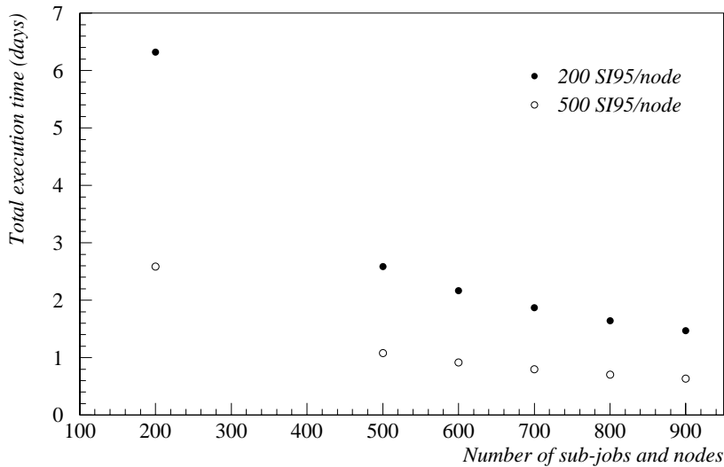
Figure 5: Execution time for full simulation at the Tier1.
