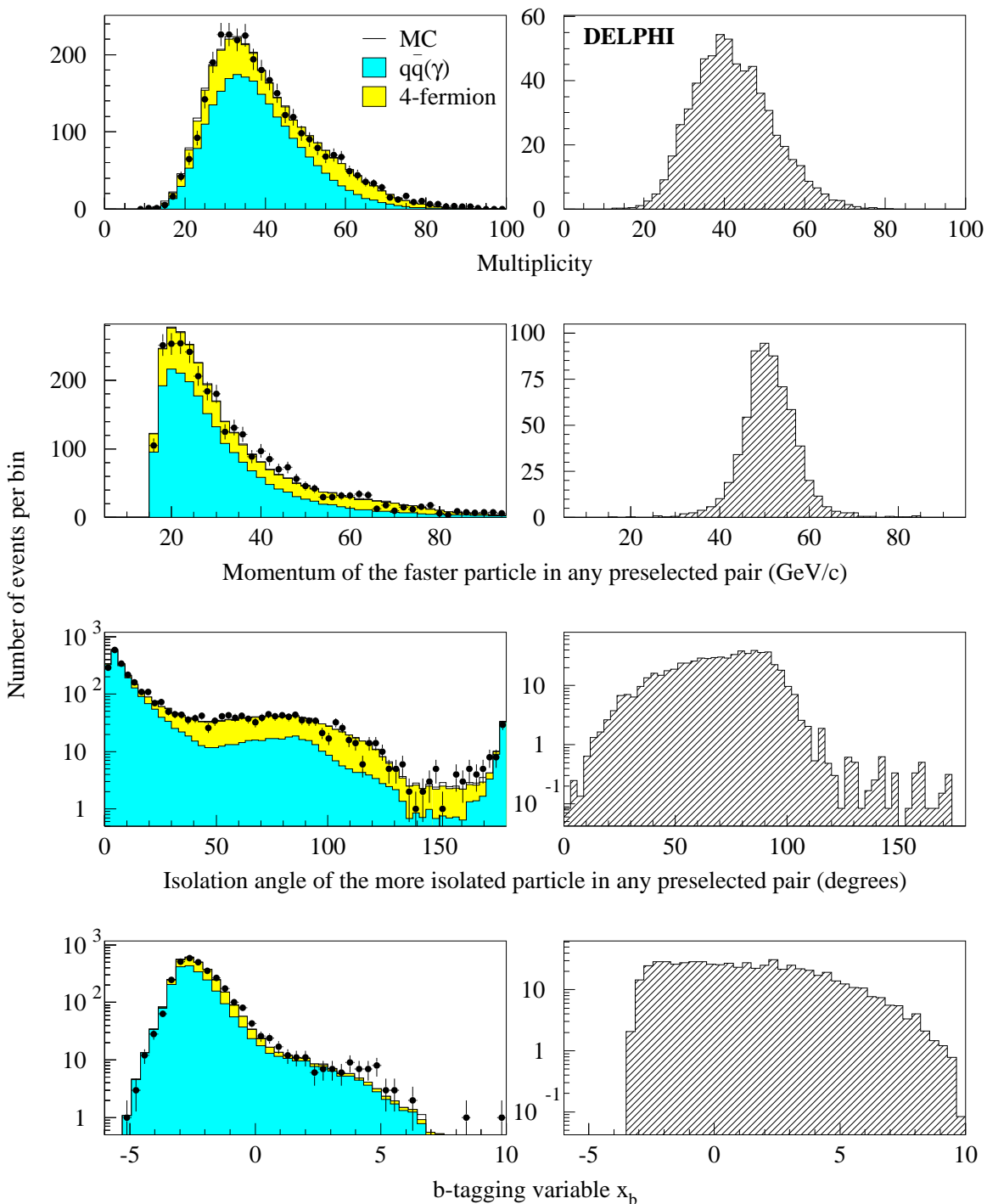
Figure 3: H\mu^+\mu^- channel: distributions of four analysis variables, as described in the text, at preselection level. Data at \sqrt{s} = 191.6\text{--}201.7 GeV (dots) are compared with SM background expectations (left-hand side histograms) and with the expected distribution for a 105 \text{ GeV}/c^2 signal (right-hand side histogram, normalised to one thousand times the expected rate).
