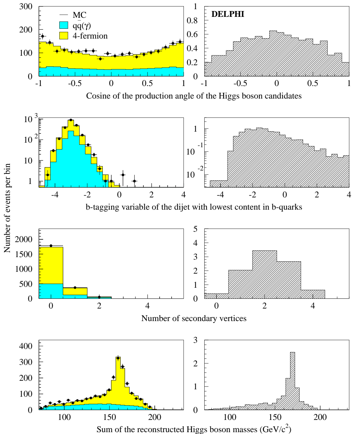
Figure 9: hA hadronic channel: distributions of four analysis variables, as described in the text, at preselection level. Data at \sqrt{s} = 191.6\text{-}201.7 GeV (dots) are compared with SM background expectations (left-hand side histograms) and with the expected distribution for a 85 \text{ GeV}/c^2 signal at \tan\beta = 20 (right-hand side histogram, normalised to the expected rate).
