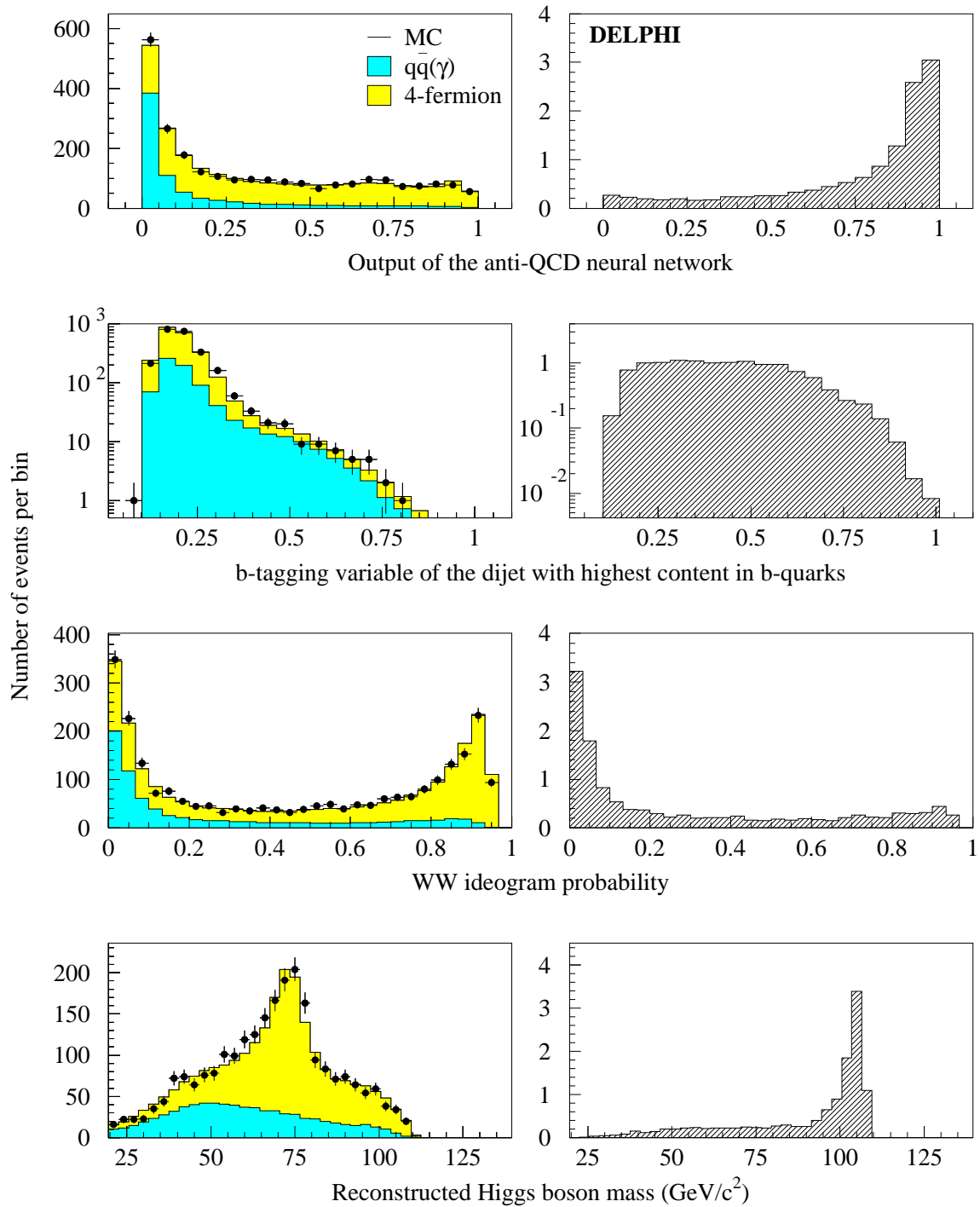
Figure 7: Hq\bar{q} channel: distributions of four analysis variables, as described in the text, at preselection level. Data at \sqrt{s} = 191.6\text{--}201.7 GeV (dots) are compared with SM background expectations (left-hand side histograms) and with the expected distribution for a 105 GeV/ c^2 signal (right-hand side histogram, normalised to the expected rate).
