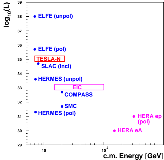
Figure 1. Luminosity versus CMS energy for existing and possible future facilities [61].
