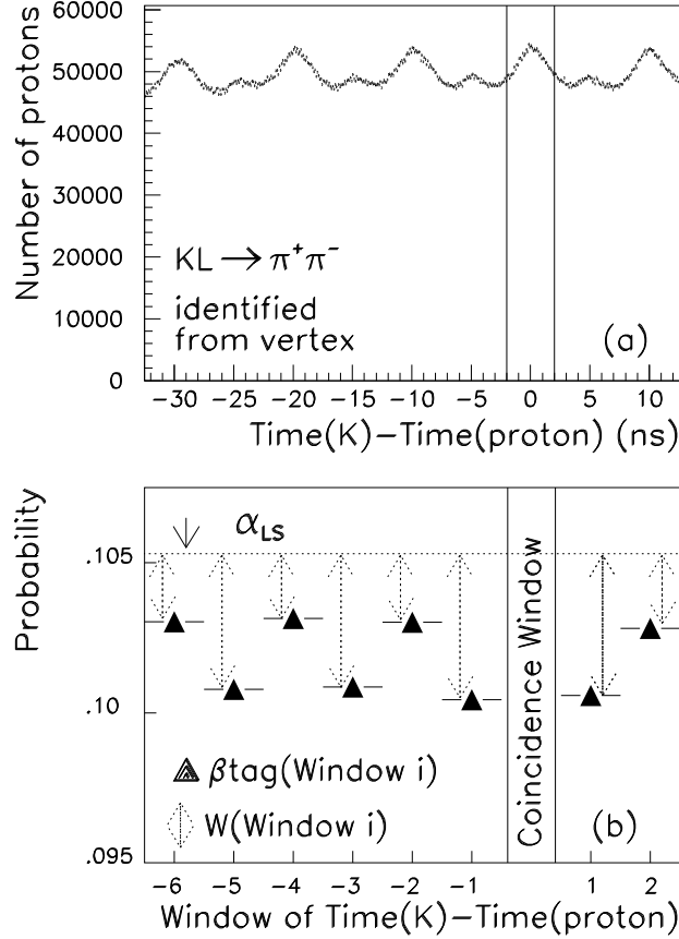
Figure 19: (a) The distribution of proton times with respect to event time for K_L \rightarrow \pi^+\pi^- identified from vertex. (b) The variables \alpha_{LS} , \beta_{tag} and W are schematically shown for K_L \rightarrow \pi\pi tagged events.
