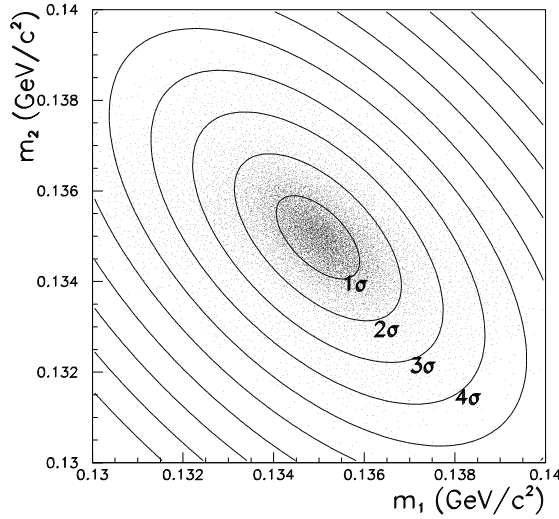
Figure 8: Distribution of K_S \rightarrow 2\pi^0 candidates in the space of two reconstructed m_{\gamma\gamma} masses, m_1 and m_2 . The contours correspond to increments by one standard deviation.
