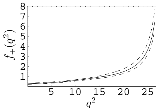
Figure 4: f_+(q^2) as function of q^2 in the entire physical range in B \rightarrow \pi e \nu , from eqs. (4.5) and (4.6), including all variations of input-parameters and M^2 . Solid line obtained from 3rd column in table 1, lower dashed curve from 2nd column and upper dashed curve from 4th column.
