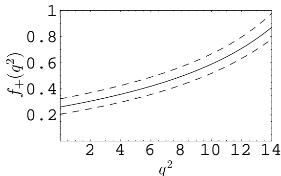
Figure 3: f_+(q^2) as function of momentum-transfer q^2 from the LCSR (4.3). Solid line: LCSR for central values of input-parameters and M^2 = 6 \text{ GeV}^2 . Dashed lines: dependence of f_+ on variation of input-parameters as specified in the text and 5 \text{ GeV}^2 \leq M^2 \leq 8 \text{ GeV}^2 .
