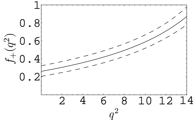
Figure 3: f_+(q^2) as function of momentum transfer q^2 from the LCSR (11). Solid line: LCSR for central values of input-parameters and M^2 = 6 \text{ GeV}^2 . Dashed lines: dependence of f_+ on variation of input-parameters as specified in the text and 5 \text{ GeV}^2 \leq M^2 \leq 8 \text{ GeV}^2 .
