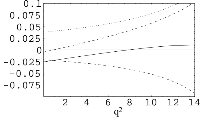
Figure 2: Radiative corrections to twist-2 and 3 contributions, in units of \alpha_s=3 , for representative input-parameters, as functions of q^2 . Dashed lines: T_H^{(p)} and T_H^{(c)} , respectively. Solid line: sum of dashed lines. Dotted line: T_H^{(2)} . The total twist-3 correction (solid line) is much smaller than the twist-2 correction (dotted line).
