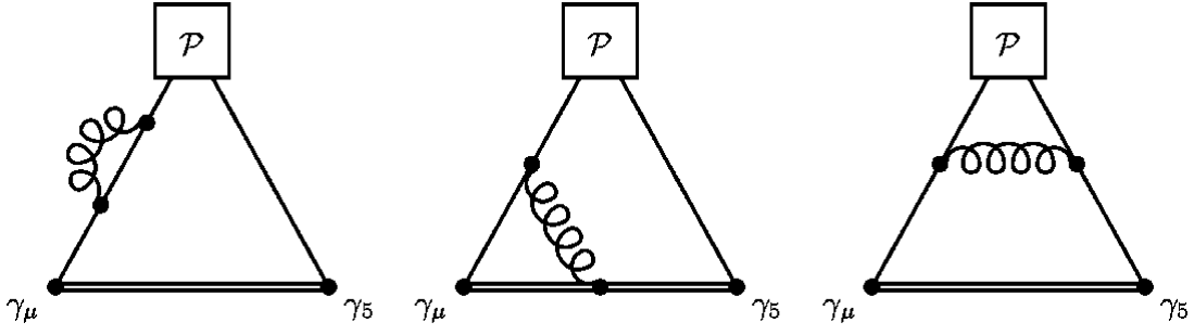
Figure 1: Some of the diagrams contributing to T_H^{(p;)} in one-loop order. The double line denotes the b-quark propagator, the single lines denote the light u- and d-quark propagators. \gamma_\mu and \gamma_5 are the weak and the B-vertex, respectively. There are two more self-energy and one more vertex-correction diagrams.
