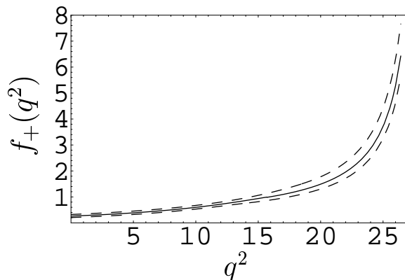
Figure 4: f_+(q^2) as function of q^2 in the entire physical range in B \rightarrow e \gamma , from Eqs. (13) and (14), including all variations of input-parameters and M^2 . Solid line obtained from 3rd column in Tab. 1, lower dashed curve from 2nd column and upper dashed curve from 4th column.
