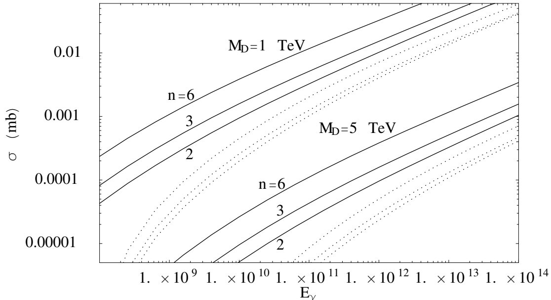
Figure 3: Cross section for black hole production as a function of E_\nu , for M_D = 1, 5 TeV and n = 2, 3, 6 . Solid and dotted lines correspond to xs > M_D^2 and xs > (10M_D)^2 respectively.
