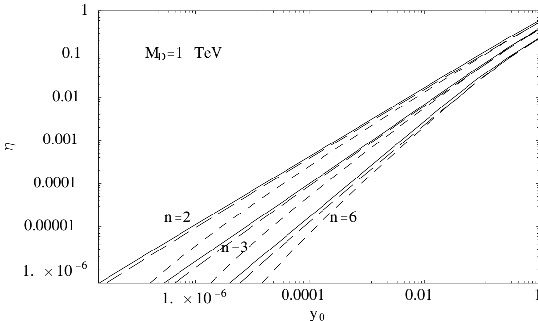
Figure 4: Fraction \eta , defined in eq. (18), of neutrino energy lost to soft scatterings. Solid, long-dashed, and short-dashed lines correspond to E_\nu = 10^{14} , 10^{12} and 10^{10} GeV, respectively.
