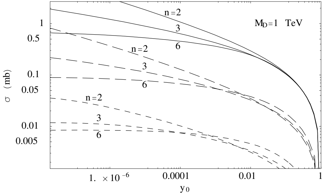
Figure 1: Elastic cross section vs. minimum fraction of energy lost by the neutrino for M_D = 1 TeV and n = 2, 3, 6 large extra dimensions. Solid, long-dashed and short-dashed lines correspond respectively to E_\nu = 10^{14} GeV, E_\nu = 10^{12} GeV and E_\nu = 10^{10} GeV.
