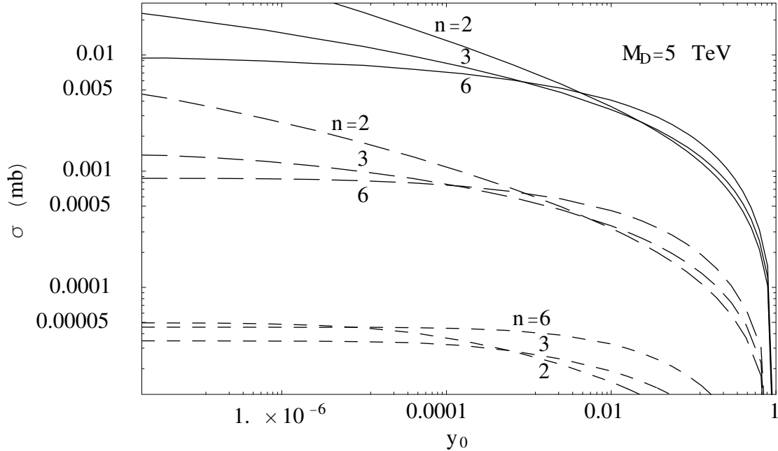
Figure 2: As in Fig. 1 but for M_D = 5 TeV.
