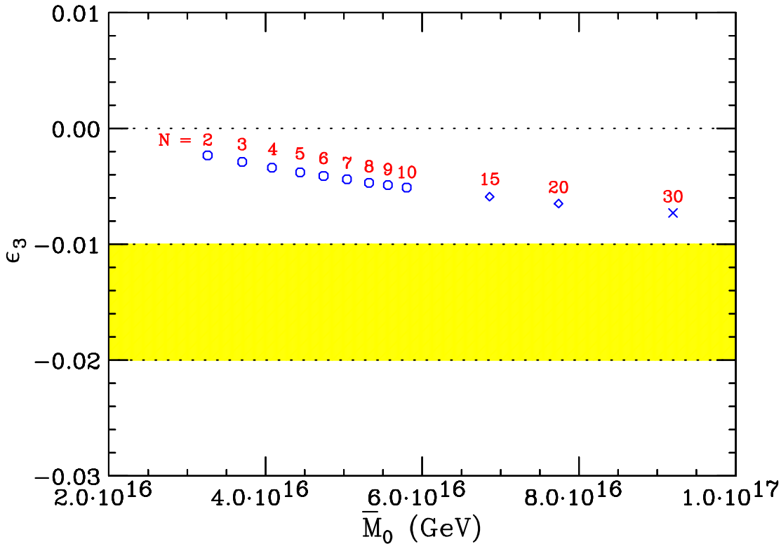
Figure 1: Predictions for \epsilon_3 and \bar{M}_0 for several different values of N . The circles (diamonds, crosses) are consistent (marginally consistent, excluded) with the proton decay limits from dimension 6 operators. The shaded region is the range of \epsilon_3 preferred by low energy data (see Eq. (3.10)).
