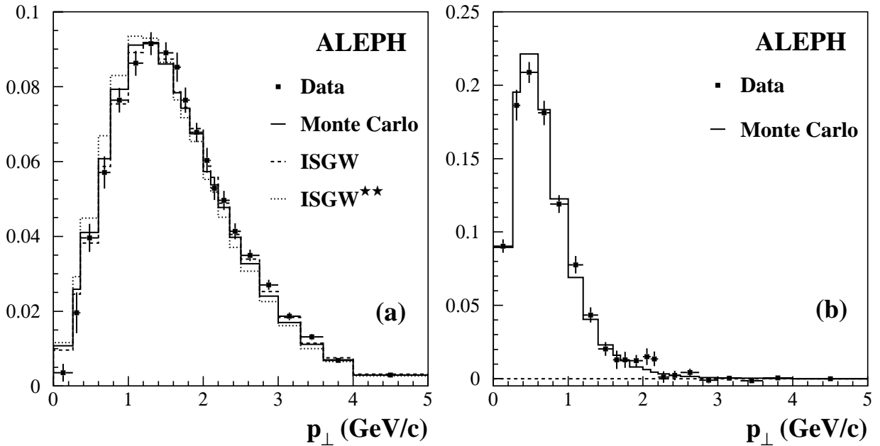
Figure 7: Comparison between the lepton p_{\perp} spectra measured in the data with the charge correlation analysis and that expected from simulation. (a) b \rightarrow Xl\nu ; data are compared with the simulation corrected as described in Section 6.15, ISGW and ISGW** models. (b) b \rightarrow c \rightarrow Xl\nu . All the spectra are normalized to unit area.
