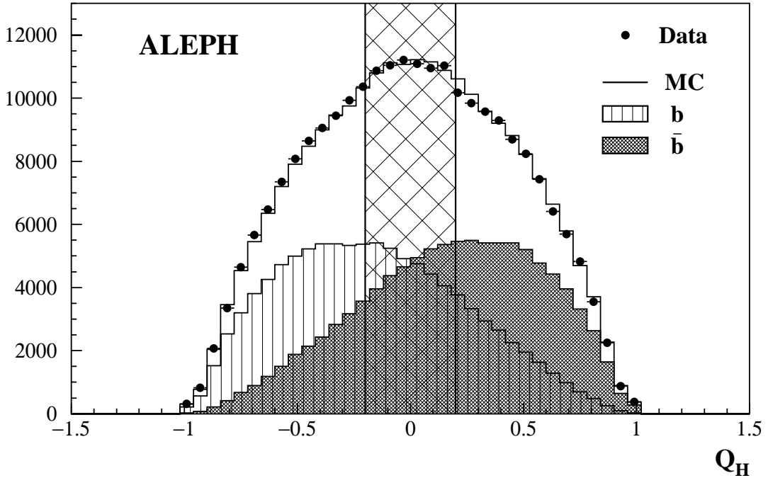
Figure 3: Distribution of the hemisphere charge estimator Q_H , in data and simulation. The contributions of hemispheres containing b and \bar{b} quarks extracted from Monte Carlo are also shown. The cross-hatched area indicates the region rejected by the selection cut.
