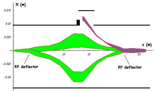
Figure 3: Beam envelopes of the bunches of Figure 2. From top to bottom: injected bunch, circulating bunches with phase \frac{2\pi}{5} and \frac{4\pi}{5} . The lines are the limits of the vacuum chamber and the rectangle stands for the injection septum.
