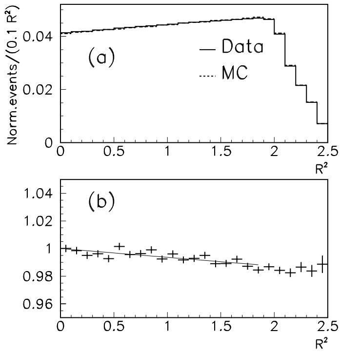
Figure 1: (a) The data (solid line) and MC (dashed line) R^2 distributions for the NUT 3\pi^0 trigger. (b) A linear fit to the normalized at R^2 = 0 ratio of these distributions.
