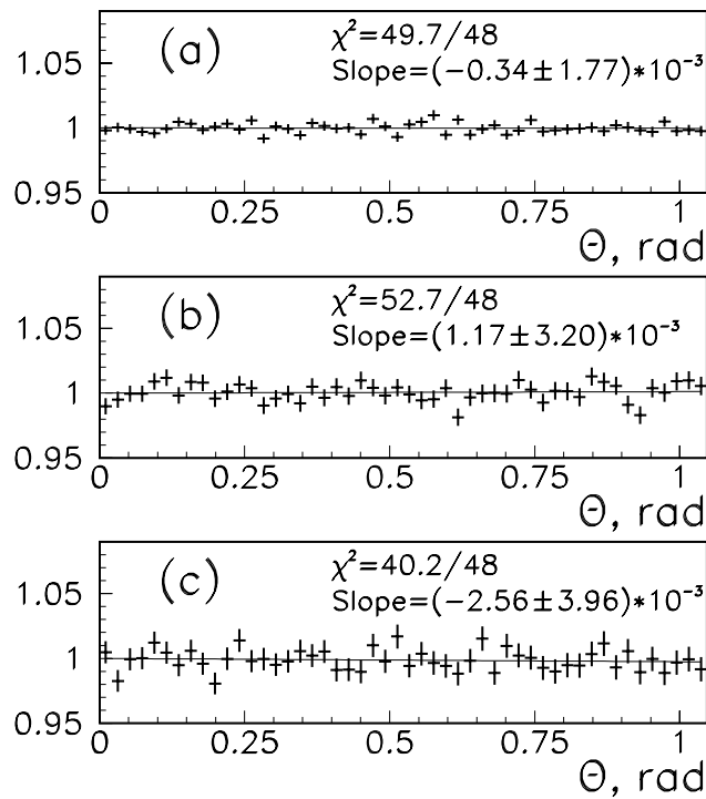
Figure 3: The normalized ratios of the data and MC \theta distributions for the NUT 3\pi^0 (a), NUT 2\pi^0 (b) and Nhodo (c) triggers. The ratios were fitted with f(\theta) = (1 + Slope \times \theta) .
