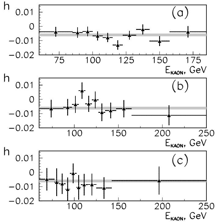
Figure 2: The K_L \rightarrow 3\pi^0 decay Dalitz plot slope parameter h in kaon energy bins for the NUT 3\pi^0 (a), NUT 2\pi^0 (b) and Nhodo (c) triggers, respectively. The overall result and the statistical error are shown by the shaded areas.
