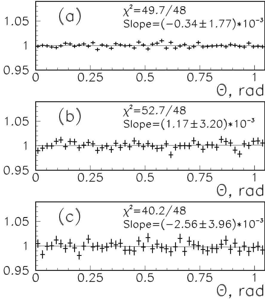
Fig. 3. The normalized ratios of the data and MC \theta distributions for the NUT 3\pi^0 (a), NUT 2\pi^0 (b) and Nhodo (c) triggers. The ratios were fitted with f(\theta) = (1 + Slope \times \theta) .
