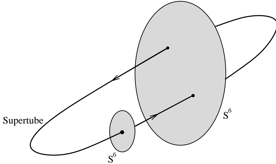
Figure 2: The little 7-disc intersects the supertube (suppressing the x -direction) at one point, hence the flux of G_4 through its boundary (the little S^6 ) is non-zero. On the contrary, the large disc intersects the supertube at two points which correspond to local D 2-brane charge densities of opposite sign, hence the flux through the large S^6 vanishes; the same happens for any 6-sphere at infinity.
