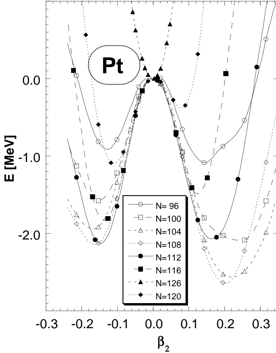
FIG. 21. Energy surface (PES) as a function of the deformation parameter \beta_2 for different isotopes of Pt.
