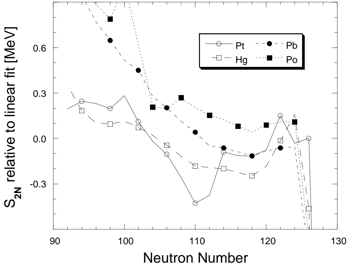
FIG. 16. Theoretical S'_{2n} values, S'_{2n}(th) , for Pt, Hg, Pb and Po using macroscopic-microscopic PES calculations.
