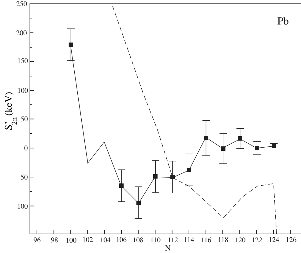
FIG. 17. S'_{2n} for Pb. Comparison between experimental data (full line connecting dots) and PES results (dashed line). The two points (N=102,104) without data point are derived, containing at least one mass value obtained from mass systematics [45].
