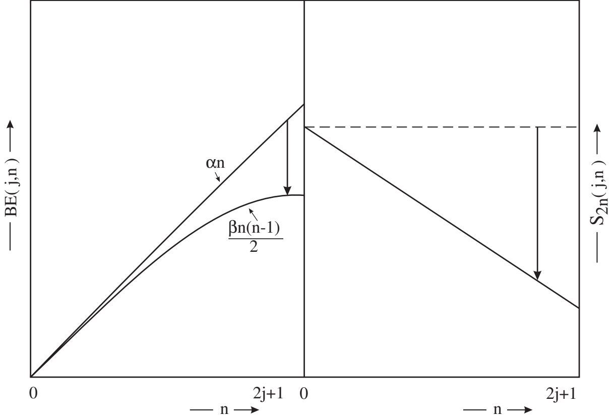
FIG. 3. Schematic representation of BE (left) and S_{2n} (right) for a shell model Hamiltonian that preserves the seniority v as a good quantum number. The two different contributions to BE ( S_{2n} ) are plotted separately.
