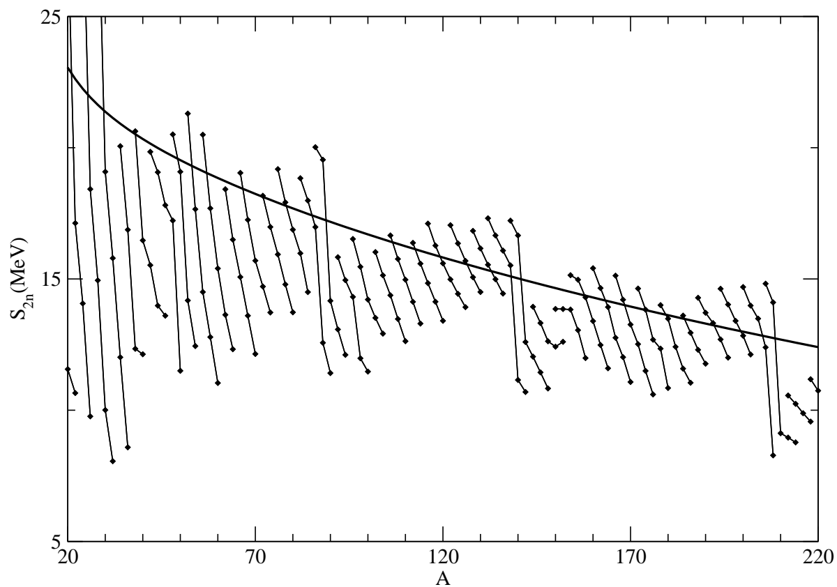
FIG. 1. Comparison between the experimental S_{2n} (diamonds) values and the LDM prediction (thick full line) along the valley of stability. The experimental data correspond to even-even nuclei around the line of maximum stability. Points connected with lines correspond to nuclei with equal Z .
