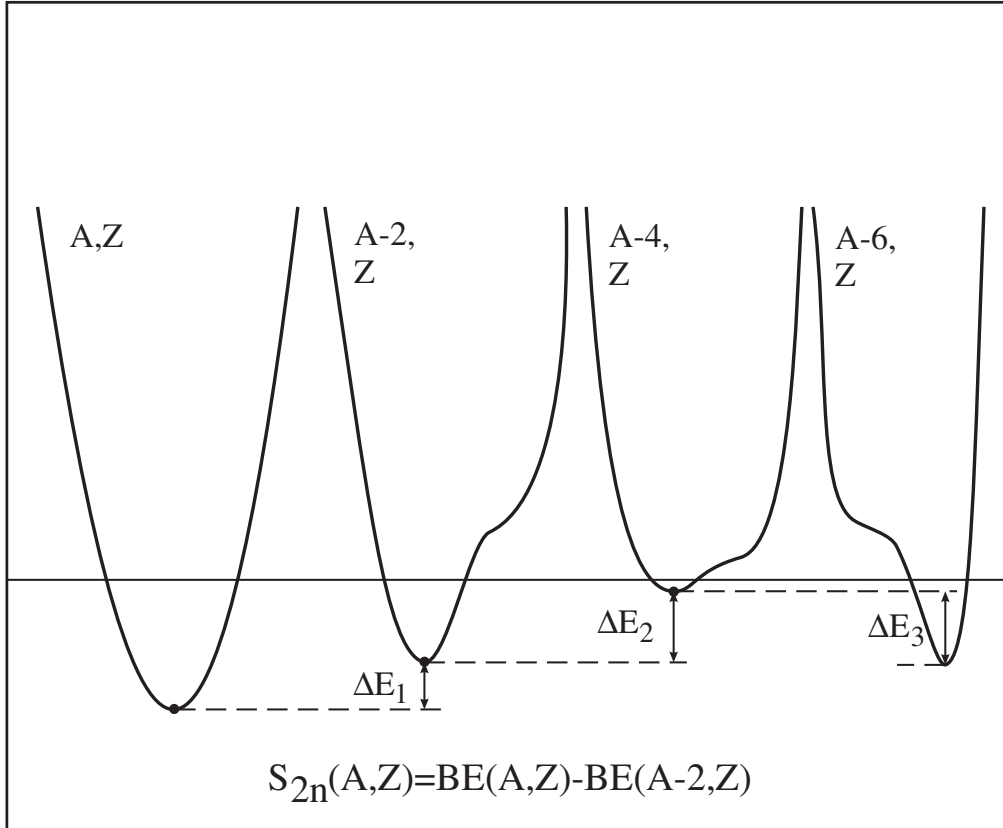
FIG. 15. Schematic representation of the method for calculating S_{2n} in the study of PES using macroscopic-microscopic models.
