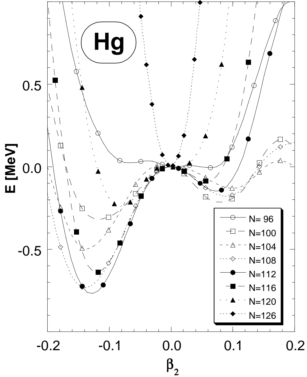
FIG. 19. Energy surface (PES) as a function of the deformation parameter \beta_2 for different isotopes of Hg.
