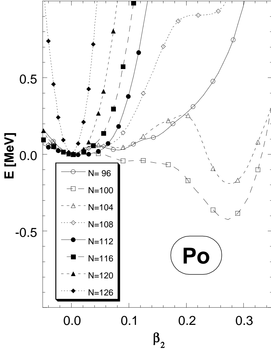
FIG. 23. Energy surface (PES) as a function of the deformation parameter \beta_2 for different isotopes of Po.
