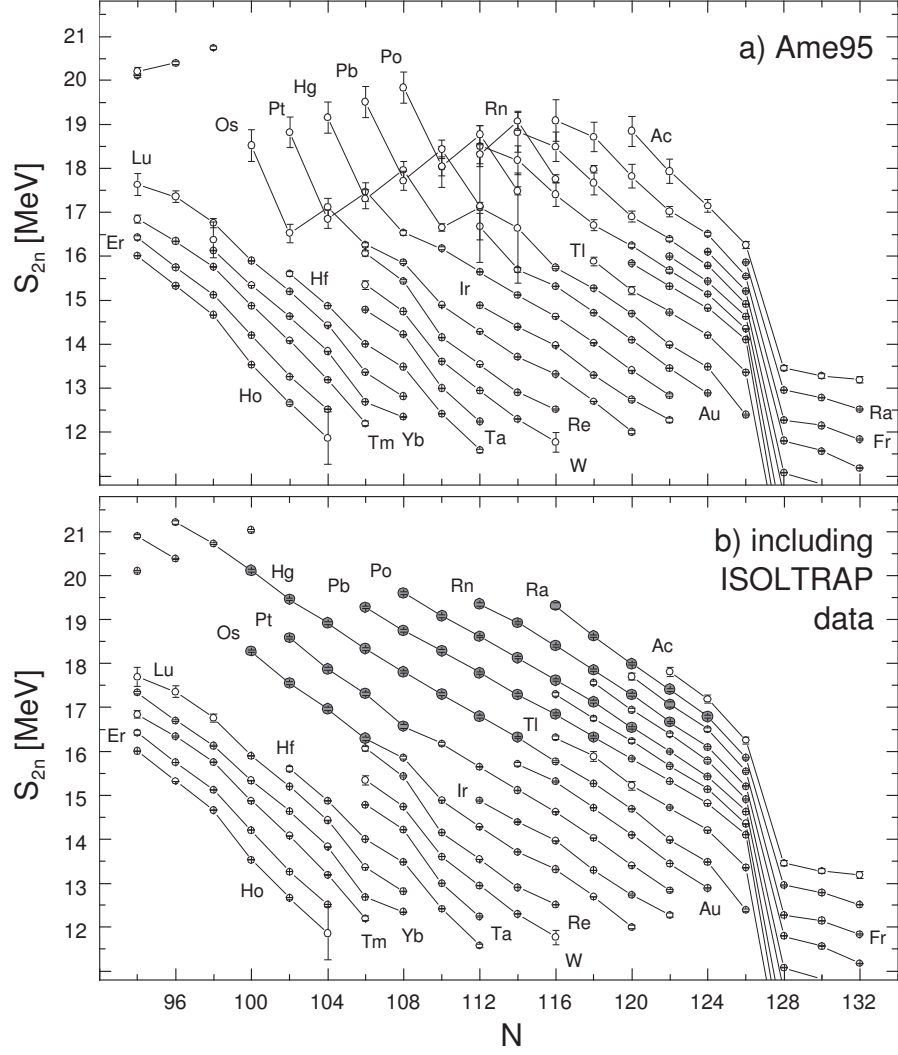
FIG. 12. Experimental two-neutron separation energies, S_{2n} , in the region of Z = 80 . a) Experimental values as determined from the analysis of Audi and Wapstra [43], including the update in 1995 [44] b) results obtained redoing the analyses of AME95, including the new ISOLTRAP data [20]. Full circles indicate S_{2n} values that are either obtained for the first time or whose errors were decreased by at least a factor two.
