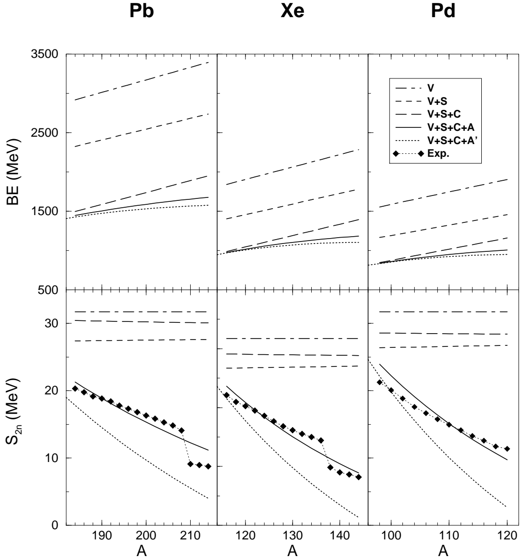
FIG. 2. Contributions of the different terms of the mass formula to the BE (top row) and S_{2n} (bottom row) for Pb, Xe, and Pd. In the S_{2n} panels are also shown the experimental data. Two different asymmetry terms are considered a_A = 23.22 MeV ( A ), full line, and a_A = 30 MeV ( A' ), dotted line.
