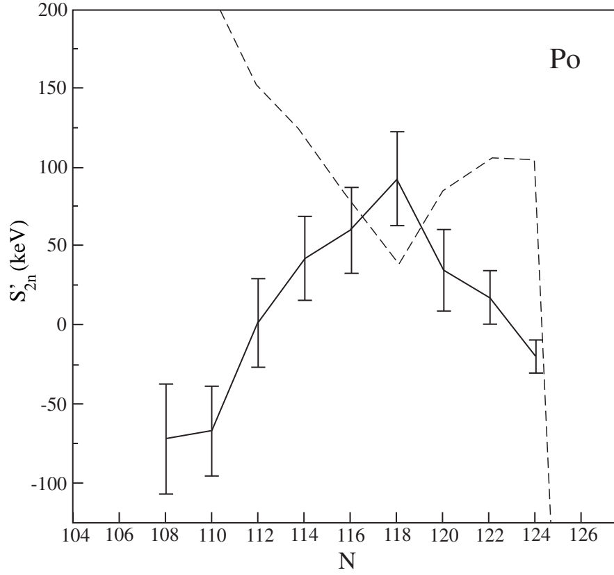
FIG. 22. S'_{2n} for Po. Comparison between experimental data (full line connecting dots) and PES results (dashed line).
