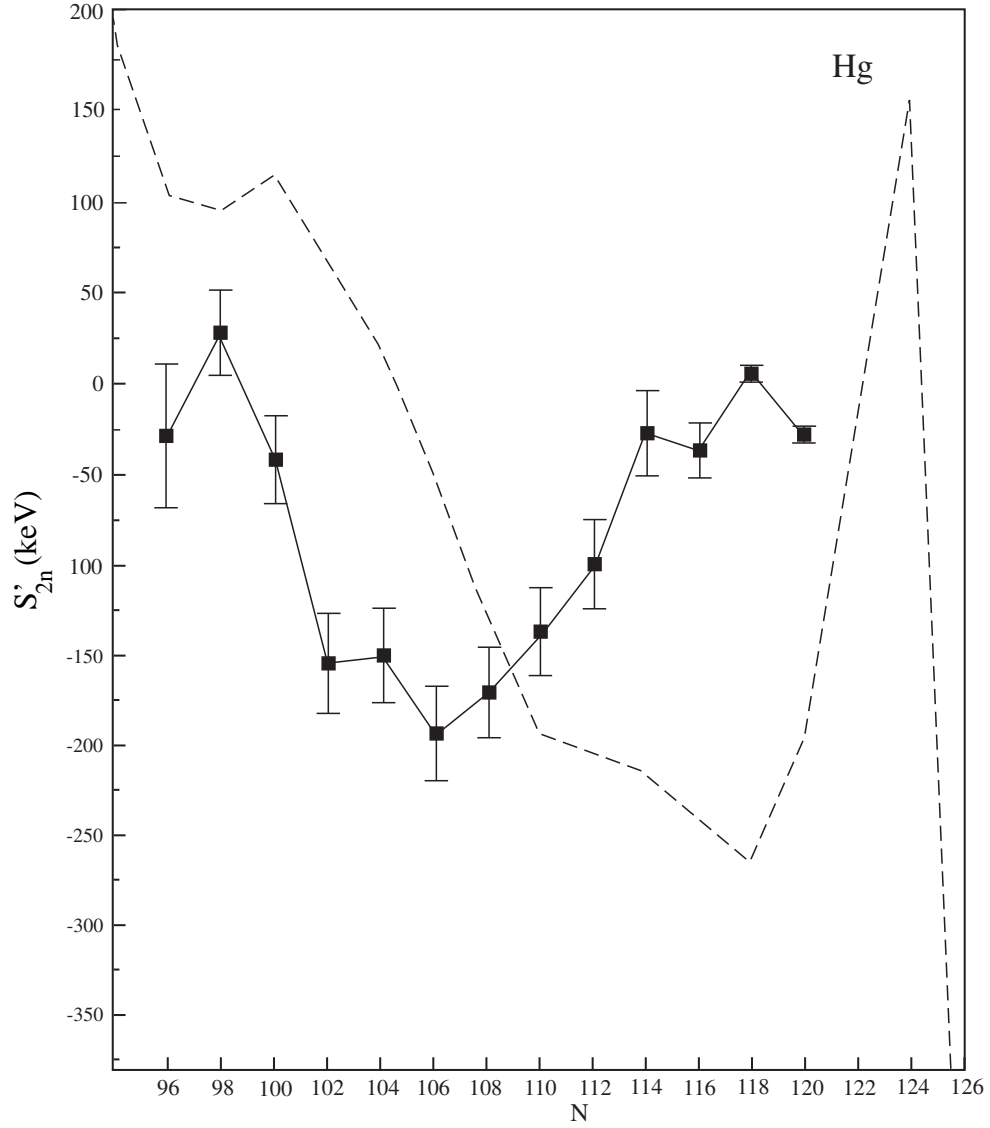
FIG. 18. S'_{2n} for Hg. Comparison between experimental data (full line connecting dots) and PES results (dashed line).
