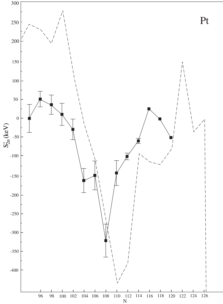
FIG. 20. S'_{2n} for Pt. Comparison between experimental data (full line connecting dots) and PES results (dashed line).
