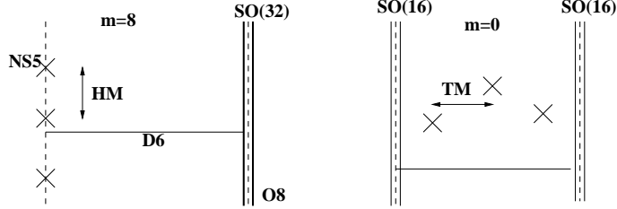
Figure 1: Examples of the two different phases in the type I' setup. Tensor multiplets correspond to motion on the compact 6 interval, hypermultiplets to motion in the transverse 789 space. The m referred to the cosmological constant set up in the bulk.
