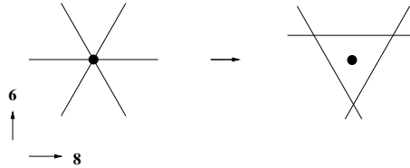
Figure 3: The 8d moduli for k=3 .
