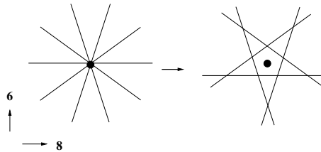
Figure 4: The 8d moduli for k=5 . The two kinds of intersections lead to two hypermultiplets.
