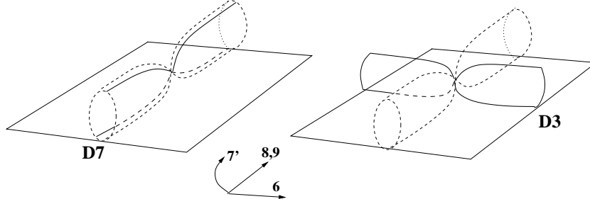
Figure 6: The 2-cycles in the Taub-NUT geometry, for D7/O7 and for D3 branes.
