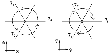
Figure 2: On the covering space the orbifold acts on the branes/planes by rotation. Including all the mirror images under the orbifold action, we are required to include branes intersecting at angles.
