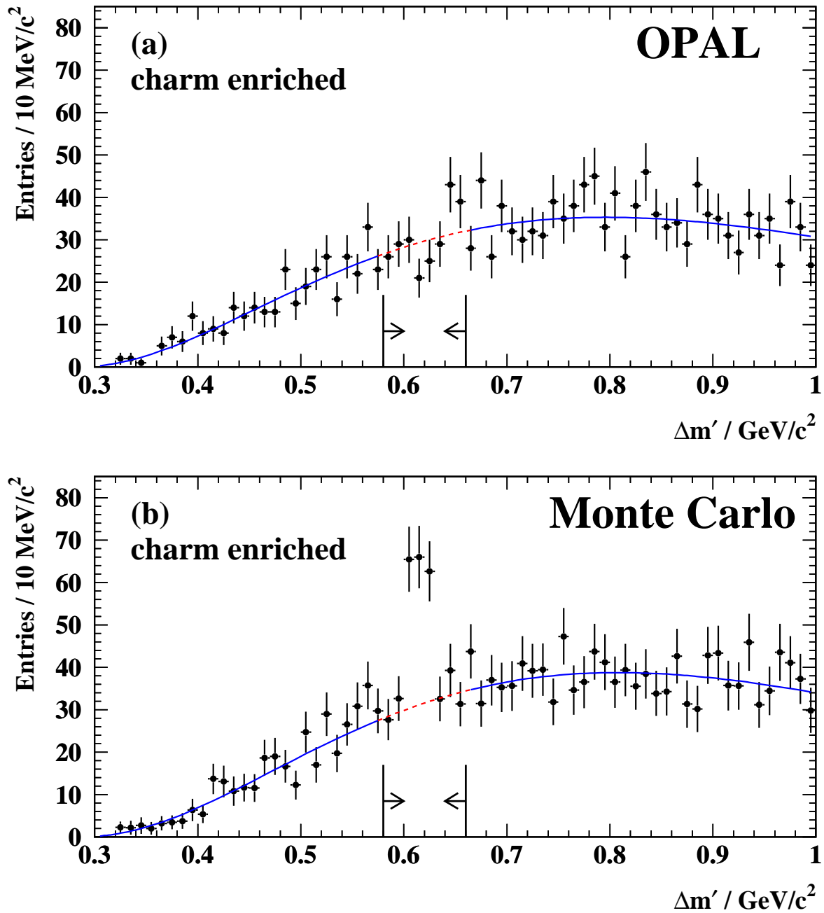
Figure 4: Distribution of the mass difference \Delta m' = m_{D^{*+}} - m_{D^{*0}} of D^{*+} candidates in the charm enriched sample, for (a) data and (b) Monte Carlo. The \chi^2/\text{dof} of the background fit is 0.80 for data, and 0.70 for the Monte Carlo simulation.
