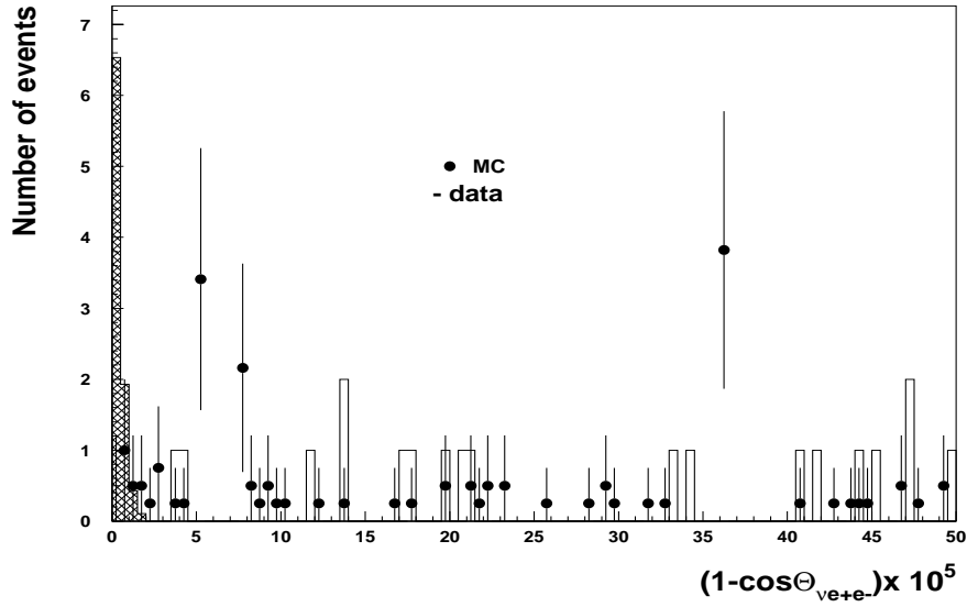
Fig. 5. The final (1 - \cos\Theta_{ve+e^-}) distribution for the data and MC. The dashed histogram represents the distribution expected from signal events.
