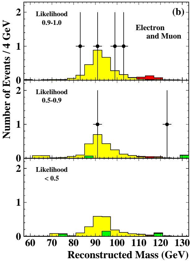
Figure 4: (a) The distribution of the variable \mathcal{D}_{mass} in the four-jet channel for a test mass of 115 GeV. (b) The reconstructed mass distribution in the electron and muon channels for the likelihood ranges of 0.9–1.0, 0.5–0.9, and range between the selection cut values (0.2 for the electron channel and 0.3 for the muon channel) and 0.5. (c) The reconstructed mass distribution in the missing-energy channel for the likelihood ranges of 0.8–1.0, 0.5–0.8, and 0.2–0.5. In all distributions, the data for \sqrt{s} \geq 204 GeV are shown with points, and the expected q\bar{q}(\gamma) backgrounds are shown with dark-shaded histograms and the expected four-fermion backgrounds are shown with light-shaded histograms. The expected distributions from a 115 GeV Higgs boson signal are shown with very dark-shaded histograms.
