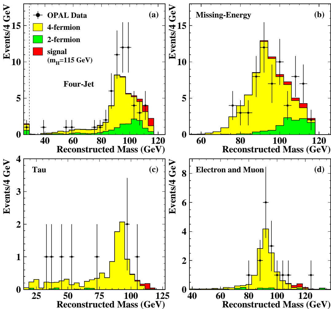
Figure 3: The reconstructed mass distribution for the selected events in the 1999 and 2000 data for (a) the four-jet channel, (b) the missing-energy channel, (c) the tau channels, and (d) the electron and muon channels combined. The first bin in (a) contains all events with \chi^2 probability of the H^0 Z^0 5C kinematic fit < 10^{-5} for chosen jet-pairings. The dark (light) grey area shows the expected contribution from the q\bar{q}(\gamma) (four-fermion) process. The Standard Model signal expectation for 115 GeV is shown with the very dark histograms on top of the Standard Model backgrounds.
