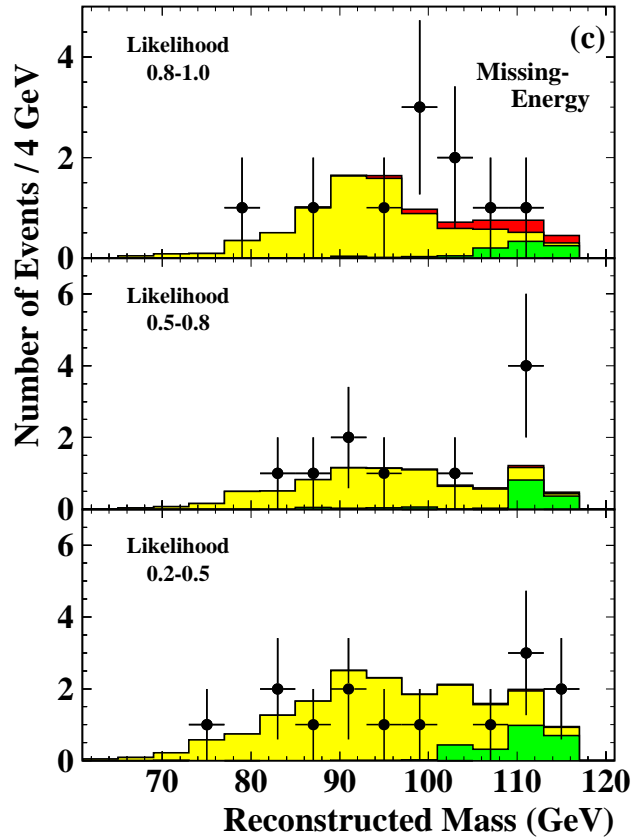
Figure 4: (a) The distribution of the variable \mathcal{D}_{mass} in the four-jet channel for a test mass of 115 GeV. (b) The reconstructed mass distribution in the electron and muon channels for the likelihood ranges of 0.9–1.0, 0.5–0.9, and range between the selection cut values (0.2 for the electron channel and 0.3 for the muon channel) and 0.5. (c) The reconstructed mass distribution in the missing-energy channel for the likelihood ranges of 0.8–1.0, 0.5–0.8, and 0.2–0.5. In all distributions, the data for \sqrt{s} \geq 204 GeV are shown with points, and the expected q\bar{q}(\gamma) backgrounds are shown with dark-shaded histograms and the expected four-fermion backgrounds are shown with light-shaded histograms. The expected distributions from a 115 GeV Higgs boson signal are shown with very dark-shaded histograms.
