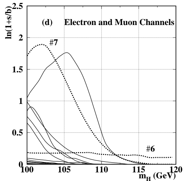
Figure 6: The \ln(1 + s/b) distributions as a function of the Higgs boson test mass for each candidate collected in 1999 and 2000 for (a) the four-jet channel, (b) the missing-energy channel, (c) the tau channels, and (d) the electron and muon channels. Each curve in the plots represents the \ln(1 + s/b) of each candidate as a function of the Higgs boson test mass. The dotted lines show the contributions of the candidates listed in Table 2.
