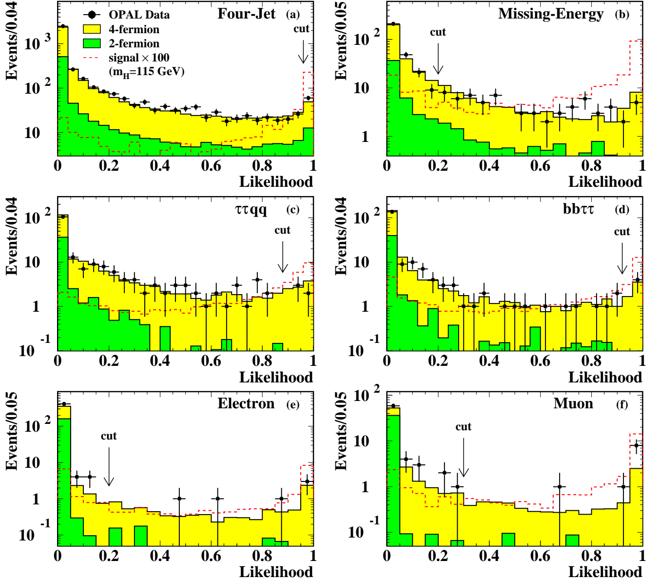
Figure 2: The distributions of the likelihood output variables in H^0Z^0 searches for the 1999 and 2000 data in: (a) the four-jet channel, (b) the missing-energy channel, (c) the tau channel \tau^+\tau^-q\bar{q} , (d) the tau channel b\bar{b}\tau^+\tau^- , (e) the electron channel and (f) the muon channel. OPAL data are shown with points, backgrounds with the shaded histograms, and the expectation from a signal with m_H = 115 GeV with the dashed histograms (scaled up by a factor of 100 for visibility.)
