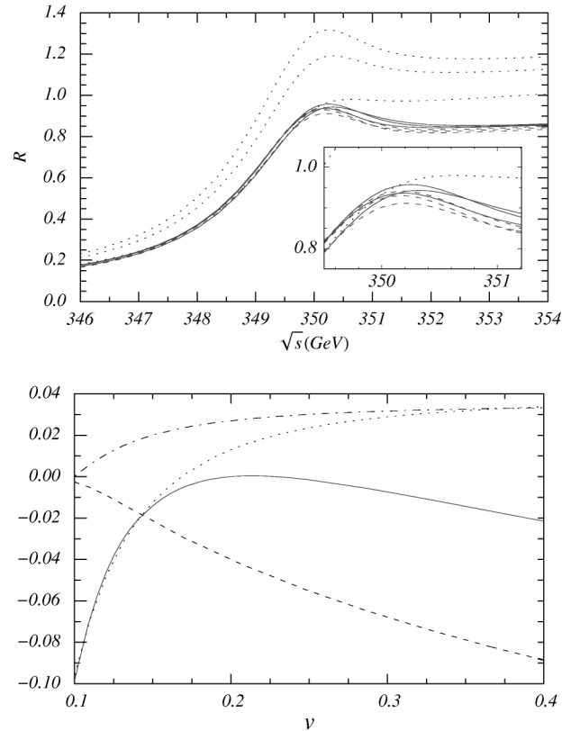
FIG. 1. The upper panel shows the normalized photon-induced cross section for t\bar{t} at LL order (dotted line), NLL order (dashed line), and NNLL order (solid line) in the 1S mass scheme with \nu = 0.15, 0.2 , and 0.4 . The lower panel shows the \nu dependence of the contributions in Eq. (15) to R^{\text{NNLL}} ( \sqrt{s} = 350 GeV). The \delta G^k contribution is shown by the dotted line, the sum of \delta G^{\delta,r,\text{kin}} terms by the dot-dashed line, the terms involving \delta G^c by the dashed line, and the sum by the solid line.
