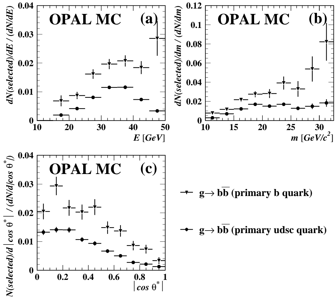
Figure 8: Selection efficiencies as a function of kinematic variables of the gluon that splits to b\bar{b} : (a) the energy E , (b) the virtuality m , (c) the decay angle |\cos\theta^*| of the b\bar{b} pair in the gluon rest-frame. The efficiencies to select q\bar{q}b\bar{b} ( q = udsc ) and b\bar{b}b\bar{b} events are indicated.
