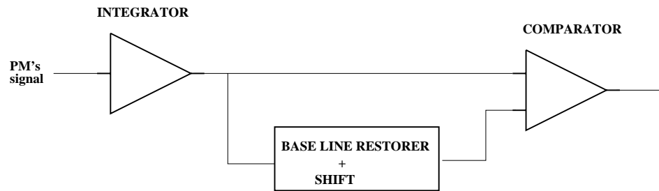
Fig. 4. Scheme of the ATC counter electronics.
