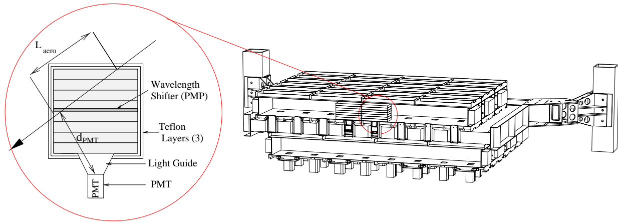
Fig. 2. View of the ATC detector design [7]. The 2 shifted layers (in x and y directions) can be seen together with the structure that allows the ATC to be directly mounted on the unique support structure. On the ATC cell view, the 8 blocks of aerogel are shown together with the 3 teflon layers and the PMP wavelength shifter lying in the middle of the cell. The impact parameter ( d_{PMT} ) used in the ATC analysis, is defined as the shortest distance between the track and the center of the PMT window (see sec. 4.4).
