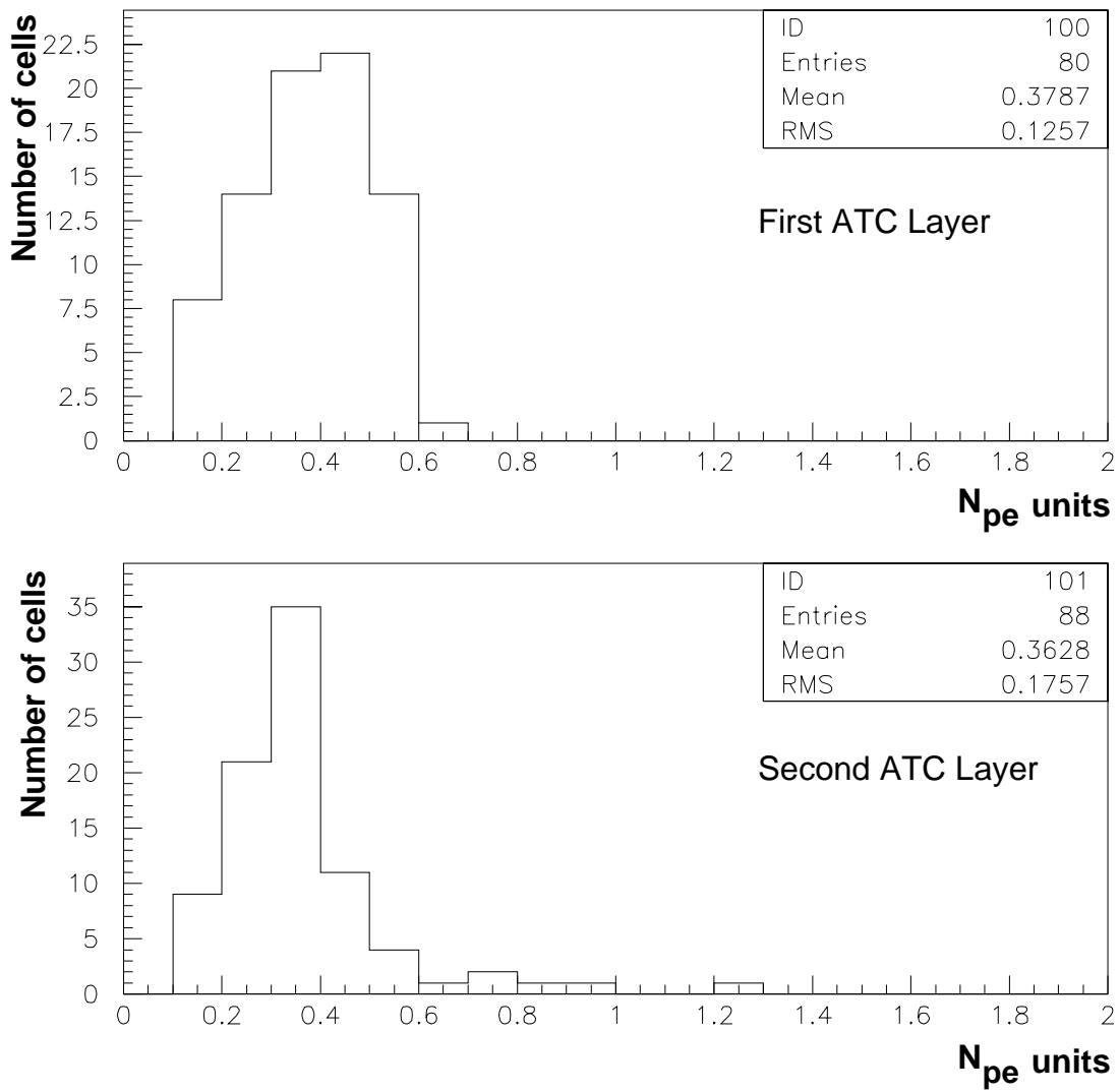
Fig. 5. Distribution of the 168 thresholds in photo-electron units, for the upper and lower ATC plane. The spreading reflects the dispersion of the PMT gains. Note that the same value of high voltage was used for a group of 16 pre-selected PMTs.
