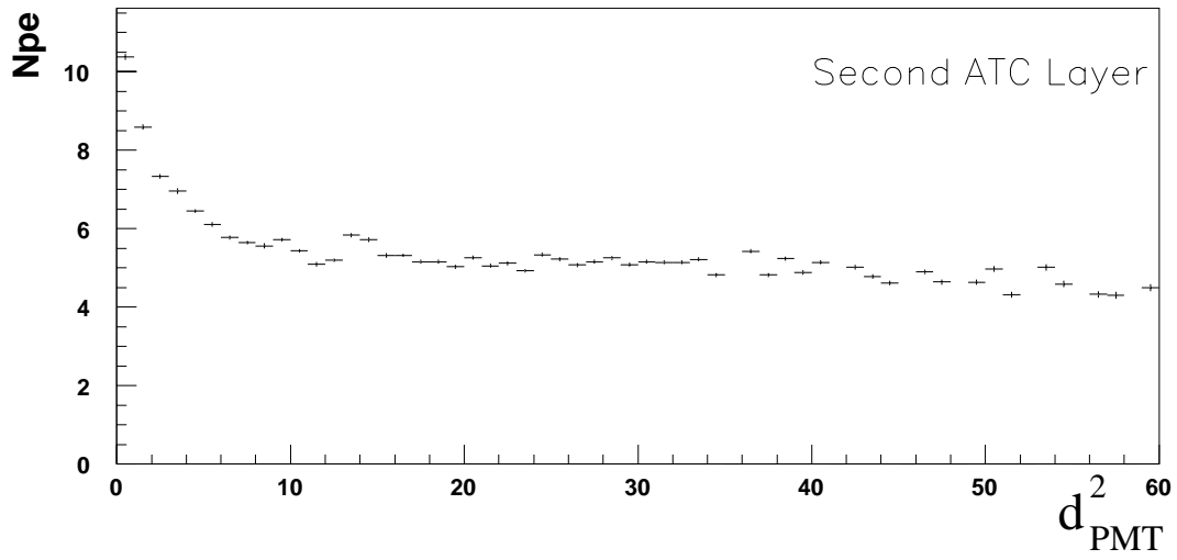
Fig. 7. Distance to PMT. The upper (lower) curve shows n_{p.e} as a function of the square of the impact parameter ( d_{PMT}^2 , in cm 2 ) for the first (second) ATC layer.
