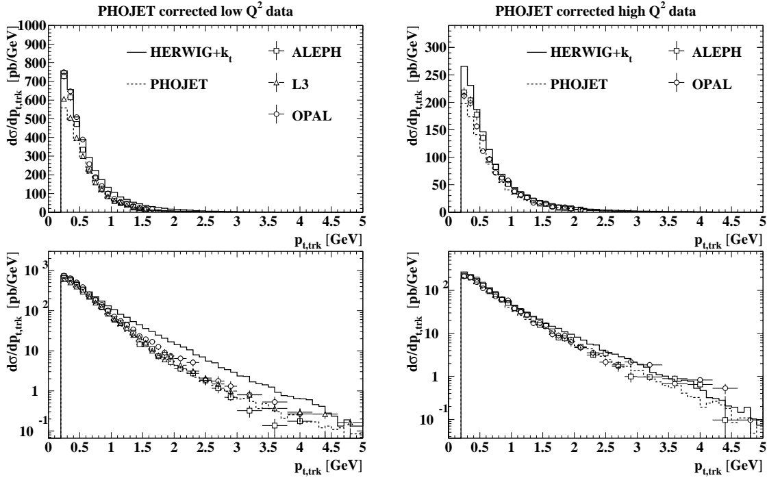
Figure 13: The p_{t,trk} distributions from ALEPH, L3 and OPAL for the low- Q^2 (left) and high- Q^2 region (right), corrected with the PHOJET model on a linear scale (top) and on a log scale (bottom).
