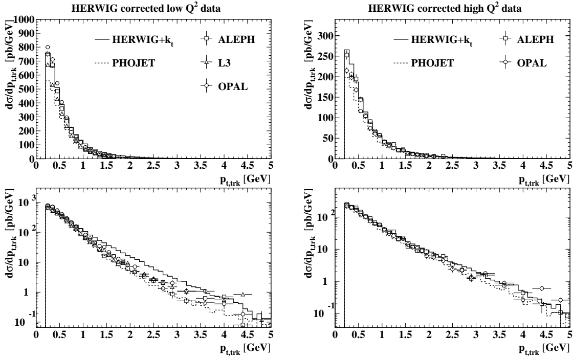
Figure 12: The p_{t,trk} distributions from ALEPH, L3 and OPAL for the low- Q^2 (left) and high- Q^2 region (right), corrected with the HERWIG+ k_t model on a linear scale (top) and on a log scale (bottom).
