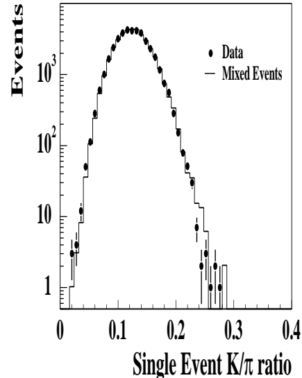
FIG. 2. Distribution of the event-by-event kaon to pion ratio estimated using a maximum likelihood method (points). As a reference, the same procedure was applied to a mixed event sample (histogram).
