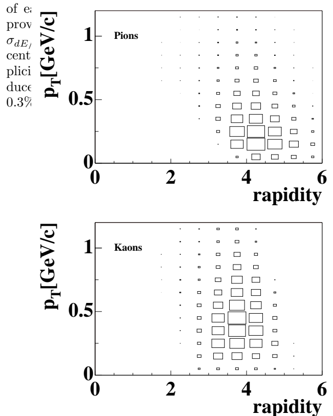
FIG. 1. Phase-space distribution of accepted charged particles pions (above) and kaons (lower plot). No acceptance correction was applied to the kaon to pion ratios reported here.
