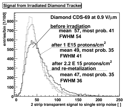
Fig. 4. Transparent 2-strip charge signal-to-noise distributions before (solid line), after proton irradiations with 1 \times 10^{15} p/cm^2 (dashed line) and after 2.2 \times 10^{15} p/cm^2 (dotted line).
