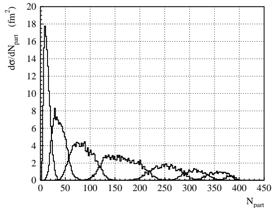
Fig. 4. Distributions of the number of participants N_{part} obtained from VENUS 4.12 for different centrality classes selected by the transverse energy E_T .
