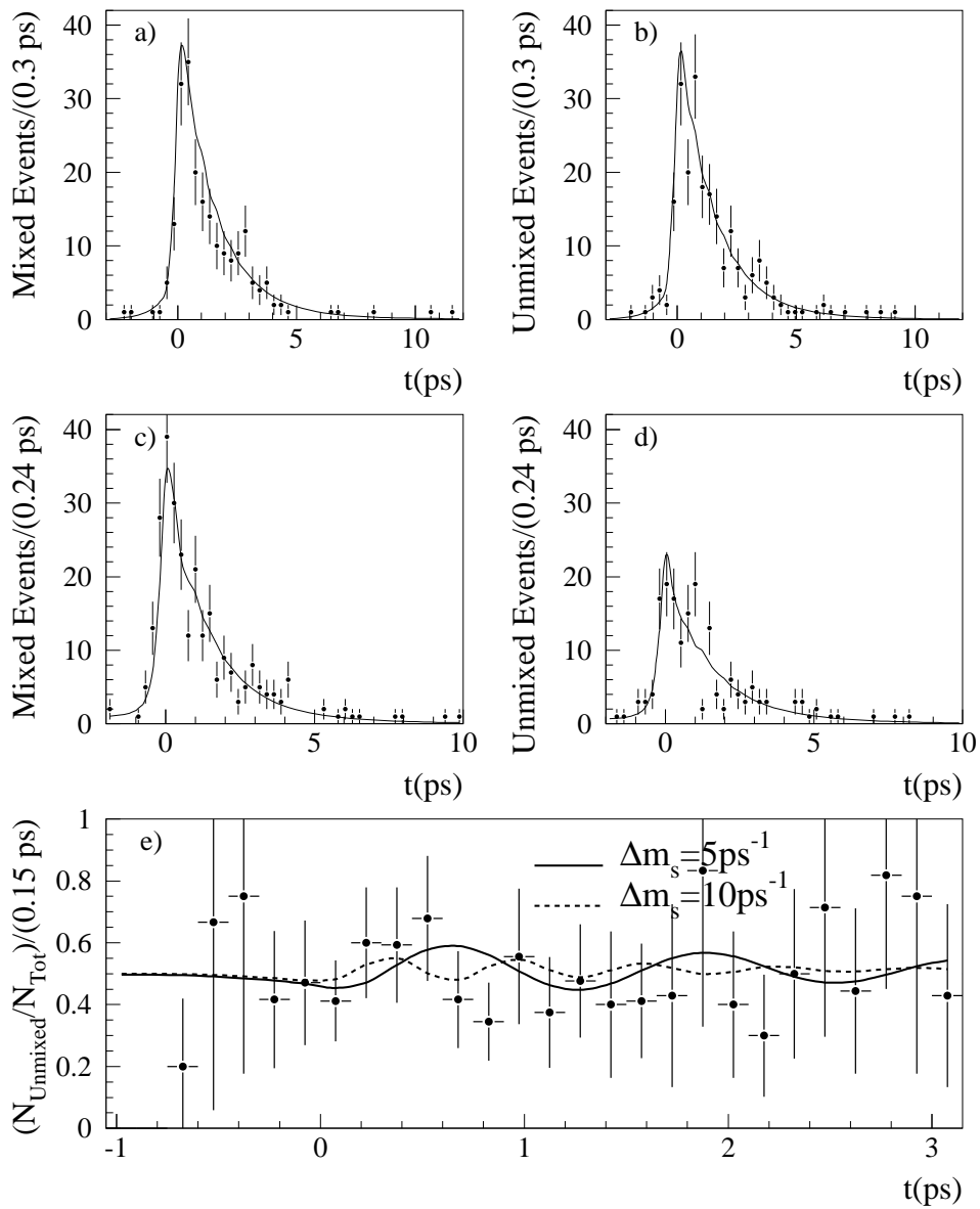
Figure 14: Proper time distribution of mixed and unmixed events in D_s l sample (a-b) and in the \phi l sample (c-d); the full dots with error bars represent the data, the curves are the corresponding distributions for \Delta m_{B_s^0} = 10 \text{ ps}^{-1} .
