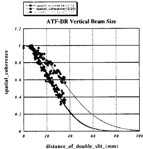
From measurements of spatial coherence, following results were obtained by orbit tuning. Once, we measured the vertical emittance of 7.5 \times 10^{-11} \text{m}^2 at the extraction line by MW1X waist scan with 50 \mu\text{m} wire (1/15/98).
