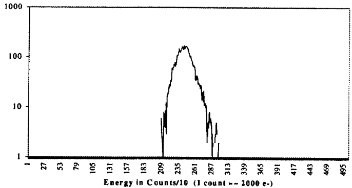
Figure 12: LED energy response for Channel 5 log scale.
