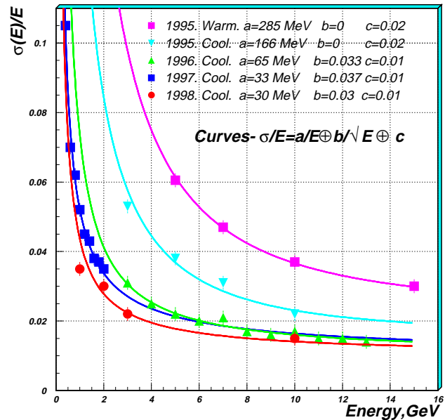
Figure 13. Summary of all beam test results for PHOS: experimental energy resolution vs. energy. The lowest curve represents the resolution requirement defined in the ALICE Technical Proposal [1].
