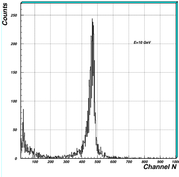
Figure 12. Spectrum from 10 GeV electrons in a PHOS 180 mm \text{PbWO}_4 crystal.
