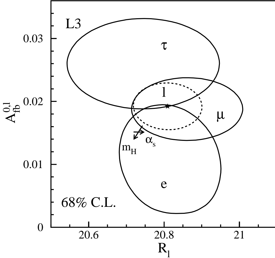
Figure 32: Contours in the A_{\text{FB}}^{0,\ell} - R_\ell plane for electrons, muons and taus obtained from a fit to total cross sections and forward-backward asymmetries. The dashed line shows the contour assuming lepton universality and the star indicates the central value. The arrows show the change in the SM prediction when varying the input parameters \alpha_s and m_H in the ranges defined in Equation 15. The uncertainty on the SM prediction due to the other parameters is small.
