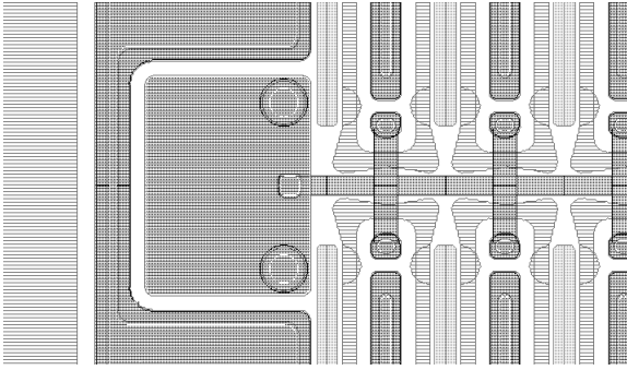
Figure 4: Details of the ST2 sensor design ( p -spray isolation) in the region of the bias grid.
