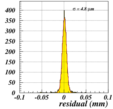
Figure 14: Distribution of the residuals for 2 pixels clusters using the binary algorithm ( 200 \mu\text{m} thick SSGb sensor).
