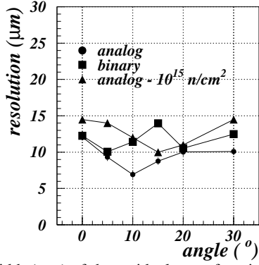
Figure 16: Width (rms) of the residuals as a function of the angle of incidence of the charged track w.r.t the normal to the sensor plane (280 \mu\text{m} thick sensors).
