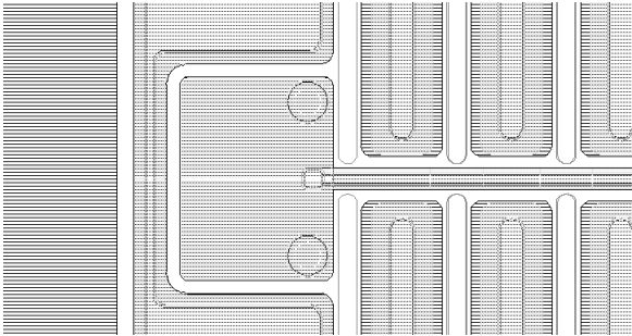
Figure 5: Details of the SSG sensor design ( p -spray isolation) in the region of the bias grid.
