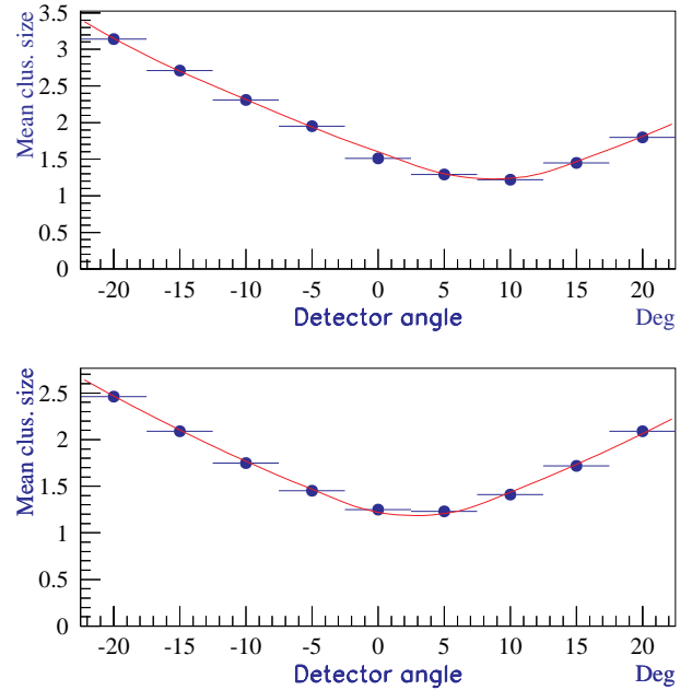
Figure 18: Mean cluster size as function of the track angle of incidence in a magnetic field of 1.4 T for a detector (top) not irradiated, (bottom) irradiated at 10^{15} \text{ n}_{\text{eq}}/\text{cm}^2 .
