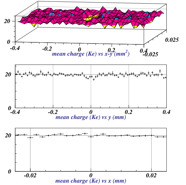
Figure 7: Average charge collected as a function of the position inside a pair of pixel cells for a 200 \mu\text{m} thick SSGb sensor.
