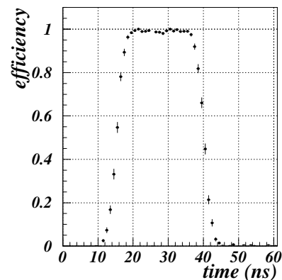
Figure 11: Efficiency versus time for a SSGb sensor.
