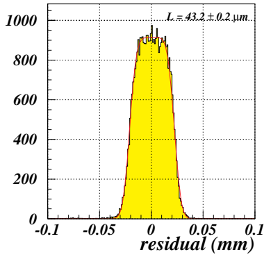
Figure 12: Distribution of the residuals for 1 pixel clusters.
