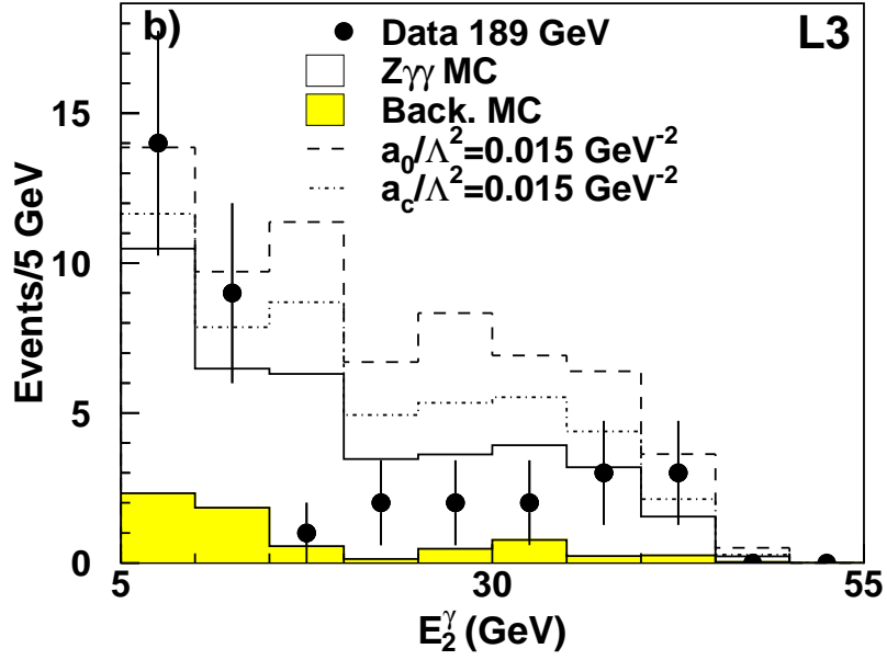
Figure 5: Energy E_2^\gamma of the least energetic photon for (a) \sqrt{s} = 183 \text{ GeV} and (b) \sqrt{s} = 189 \text{ GeV} . Data, Z\gamma and background MC are displayed together with QGC predictions.
