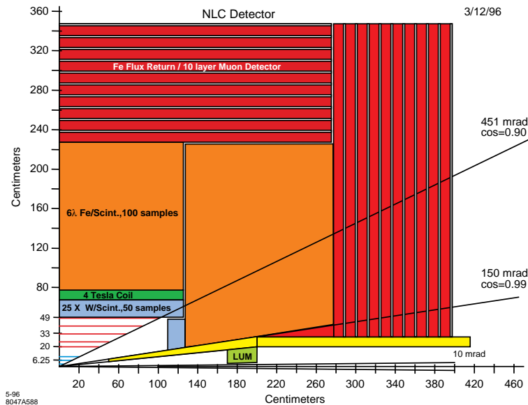
Figure 2.49: NLC Detector.
