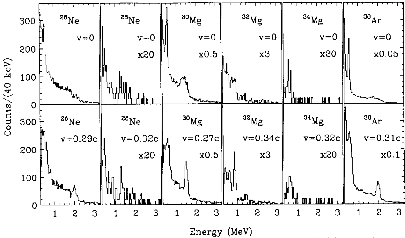
FIG. 1. Upper panels contain background subtracted photon spectra in the laboratory frame. The 547 keV ( 7/2^+ \rightarrow g.s. ) transition in the gold target is visible as a peak, while the ( 2^+ \rightarrow g.s. ) transitions in each projectile are very broad. Lower panels contain Doppler-corrected, background-subtracted \gamma -ray spectra.
