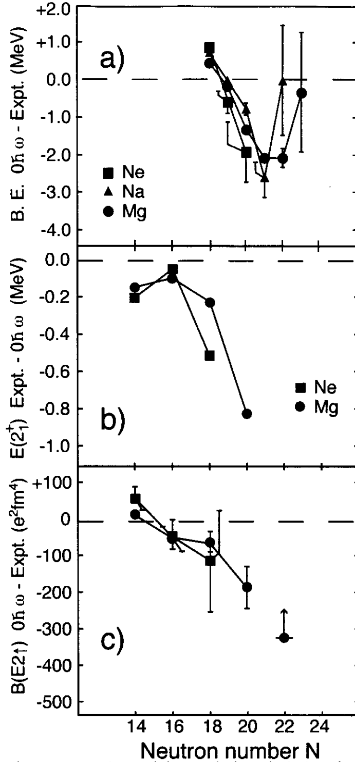
FIG. 2. Differences between experimental data and 0\hbar\omega calculations for (a) binding energies in Ne, Na and Mg isotopes; (b) energies of 2_1^+ states in Ne and Mg isotopes; and (c) B(E2; 0_{gs}^+ \rightarrow 2_1^+) values in Ne and Mg isotopes.
