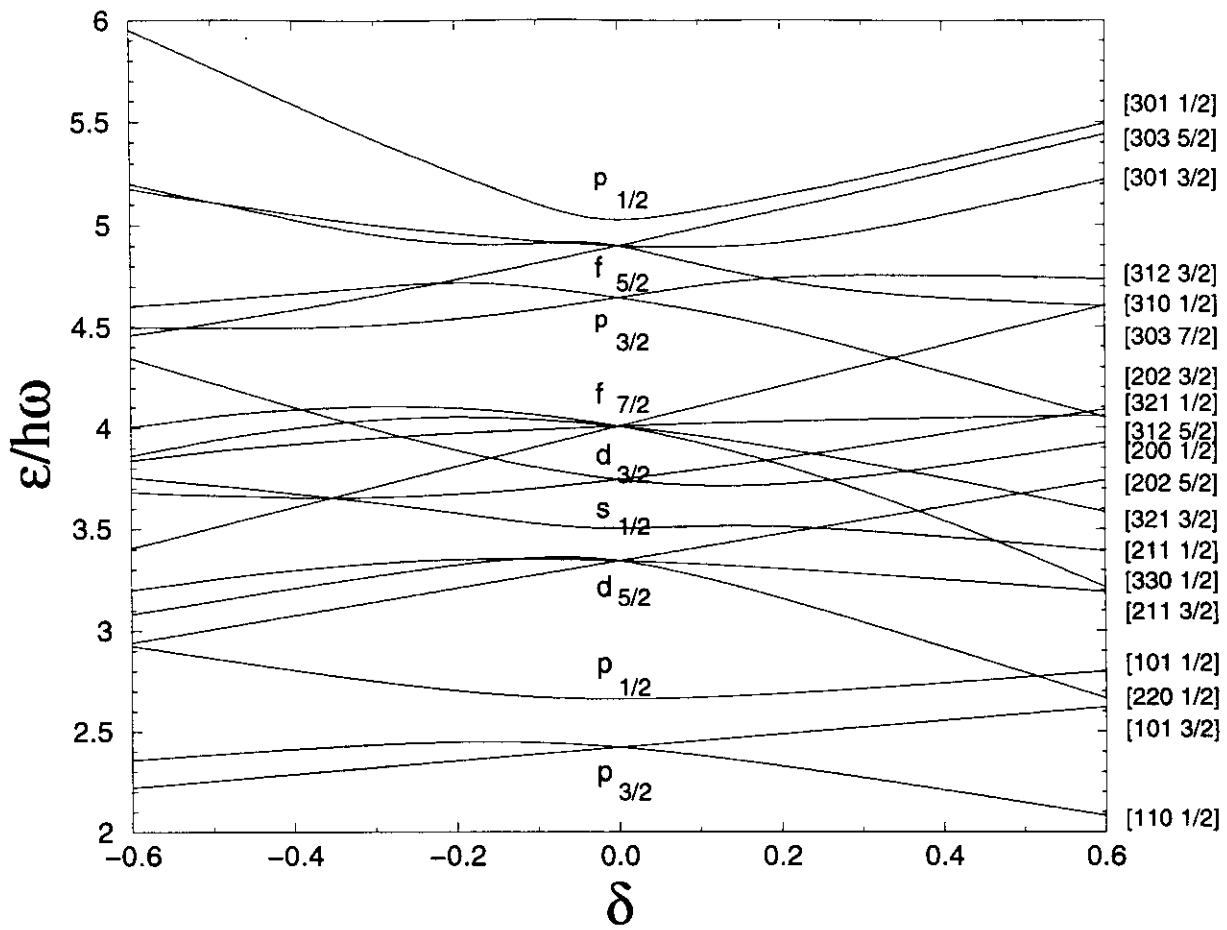
FIG. 3. The Nilsson model diagram used for the calculations described in the text.
