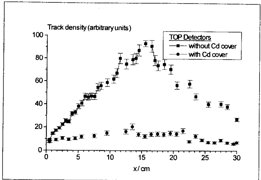
Fig.14. Thermal (without Cd cover) and epithermal (with Cd cover) neutrons detected on top of the moderator with LR-115- II B SSNTD [24] as observed in the reaction 7.4 \text{ GeV } p + \text{Pb}
