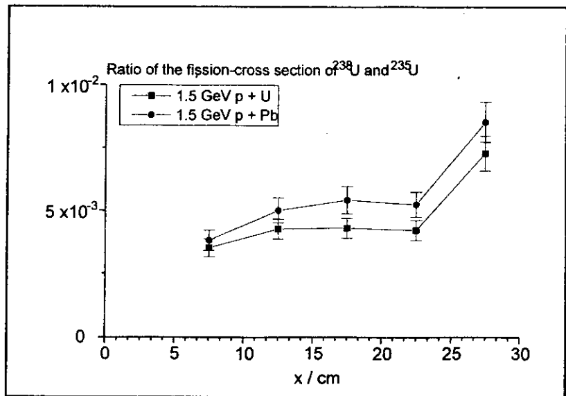
Fig.15. Ratio S of the cross-section for the fission of ^{238}\text{U} and ^{235}\text{U} on top of the moderator during the Pb- and U-targets [25] experiments with 1.5 GeV protons
