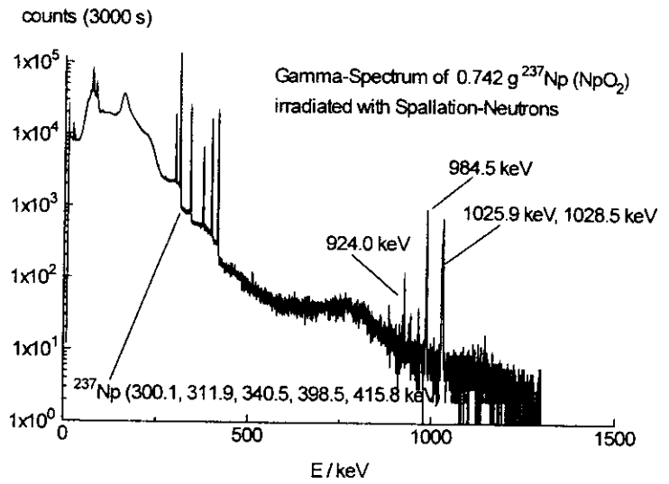
Fig. 5. Spectrum of ^{237}\text{Np} irradiated with spallation neutrons from an U target (7.4 GeV p) hielded with 1cm Pb: ^{238}\text{Np} (924, 984, 1026, 1028 keV)
