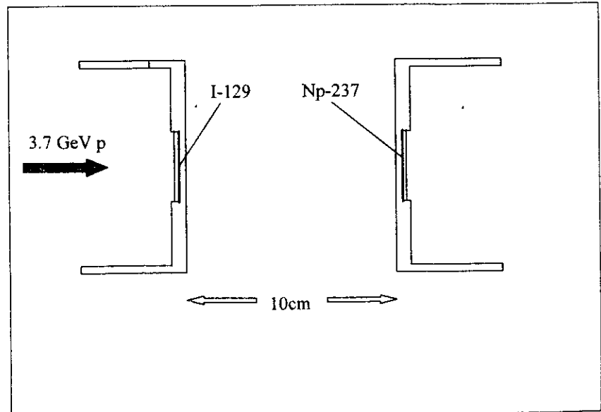
Fig. 4. Setup for the direct irradiation of ^{129}\text{I} and ^{237}\text{Np} with 3.7 GeV protons
