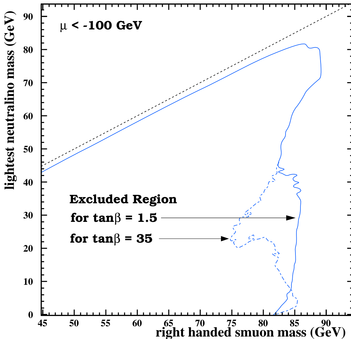
Figure 15: For two values of \tan\beta and \mu < -100 \text{ GeV} , 95% CL exclusion regions for right-handed smuon pairs within the MSSM, obtained by combining the \sqrt{s} = 183 and 189 \text{ GeV} data-sets. The excluded regions are calculated taking into account the predicted branching ratio for \tilde{\mu}_R^\pm \rightarrow \mu^\pm \tilde{\chi}_1^0 . The gauge unification relation, M_1 = \frac{5}{3} \tan^2 \theta_W M_2 , is assumed in calculating the MSSM branching ratios. The kinematically allowed region is indicated by the dashed line.
