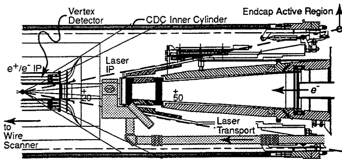
Figure 1. Cutaway elevation view of the inside of the SLD. The new vertex detector [10], surrounding the e+/- IP with the wire scanner on one side (not shown) and the laser profile monitor on the other, is itself surrounded by the 13 inch inner cylinder of the SLD central tracking drift chamber (CDC). Access is not available beyond a few inches from the end of the cylinder. The laser transport line (shaded) enters from the bottom right of the figure and passes through two bellows before terminating in the IP optics bench. The numbers along the central axis indicate the distance in cm from the e+/- IP.
