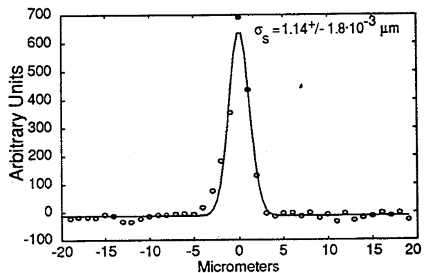
Figure 4. A typical profile monitor scan showing \sigma_s . The horizontal scale is determined using the transfer matrix ( R_{34} ) for the scan coils to the laser IP. The collision signal in this case is detected using the SLD polarimeter degraded e- detector, located after the first large bend in the outgoing beamline. Each data point is the average of 3 beam pulses with the laser on, with the average of 6 pulses with the laser off subtracted.
