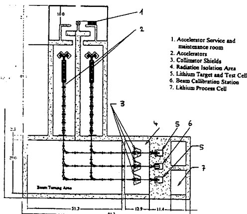
Fig. 5 IFMIF general lay out
