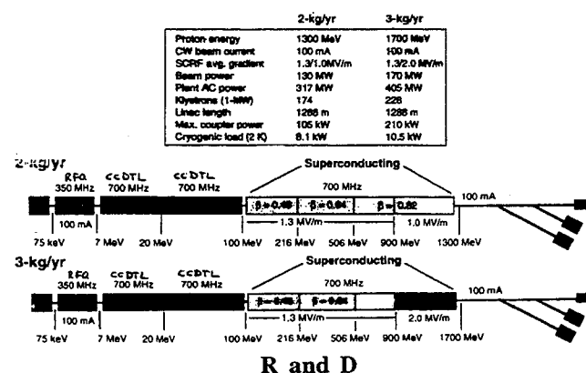
Fig. 8 APT superconducting linac.
