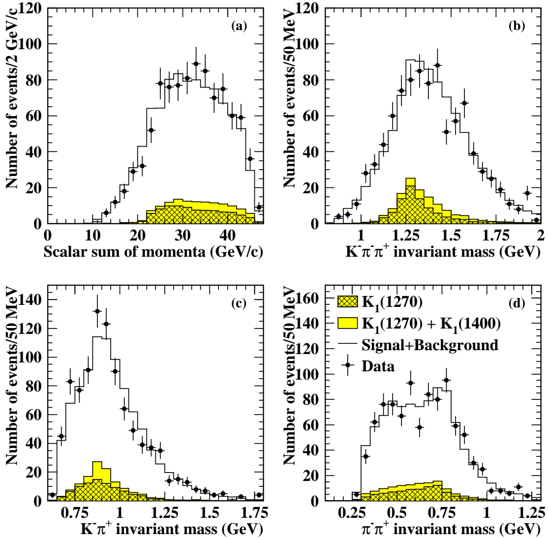
Figure 6: (a) is the \Sigma P distribution and (b), (c), and (d) are the invariant mass distributions of the data \tau^- \rightarrow \nu_\tau K^- \pi^- \pi^+ candidate sample (points). The histogram represents the predicted distribution, in which the normalisation of the background and signal components comes from the best fit results of the binned maximum likelihood fit which took the correlations between the invariant mass distributions into account. The shape of the signal is estimated using \tau^- \rightarrow \nu_\tau K^- \pi^- \pi^+ events generated through the \text{K}_1(1270) and the \text{K}_1(1400) resonances, where the widths of the resonances are taken to be 90 and 174 MeV, respectively [14]. The shape of the \tau^- \rightarrow \nu_\tau \pi^- \pi^- \pi^+ (\pi^0) background in the distributions is obtained from a data control sample.
