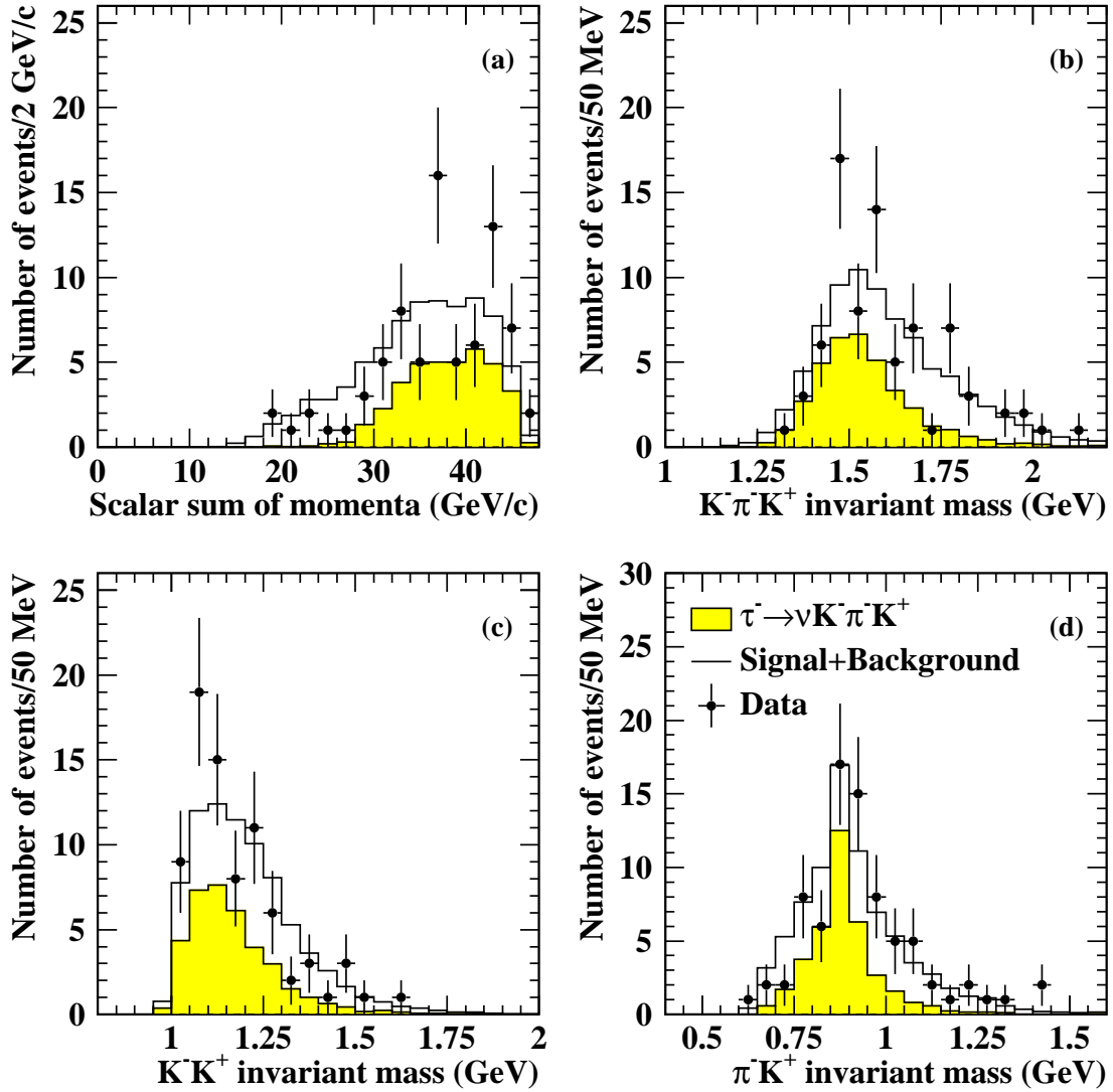
Figure 7: (a) is the \sum P distribution and (b), (c), and (d) are the invariant mass distributions of the data \tau^- \rightarrow \nu_\tau K^- \pi^- K^+ candidate sample (points). The histogram represents the predicted distribution, in which the normalisation of the background and signal components comes from the results of the binned maximum likelihood fit to the four distributions. The shape of the \tau^- \rightarrow \nu_\tau K^- \pi^- K^+ signal distribution is simulated in the fit by Monte Carlo events generated by the default version of Tauola 2.4. The shape of the \tau^- \rightarrow \nu_\tau \pi^- \pi^- \pi^+ (\pi^0) background in the distributions is obtained from a data control sample.
