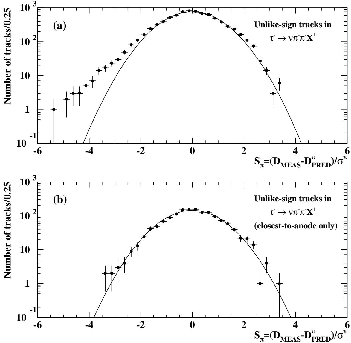
Figure 2: (a) is the stretch dE/dx distribution under the pion hypothesis for the unlike-sign tracks in the data \tau^- \rightarrow \nu_\tau \pi^- \pi^- X^+(\pi^0) candidate sample (points). This sample is expected to have less than three kaons present. The curve is a unit width Gaussian of zero mean, whose normalisation is fit to the central part of the distribution. A significant non-Gaussian component is evident. (b) is the same distribution for the unlike-sign tracks in the data first-track \tau^- \rightarrow \nu_\tau \pi^- \pi^- X^+(\pi^0) candidate sample.
