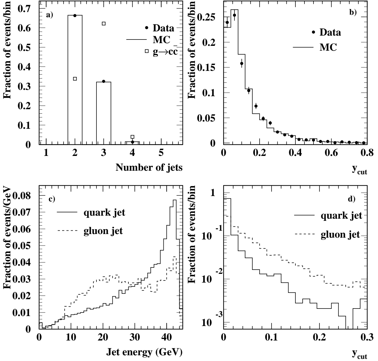
Figure 1: Jet selection properties: a) number of jets in the events; b) y_{cut} value where a selected jet splits into two subjets for all three-jet events; c) jet energy for quark and gluon jets in Monte Carlo g \rightarrow c\bar{c} events; d) y_{cut} value at the point where a jet splits into two subjets for quark and gluon jets. The Monte Carlo histograms in a) and b) include the default JETSET value of g_{c\bar{c}}=0.014 .
