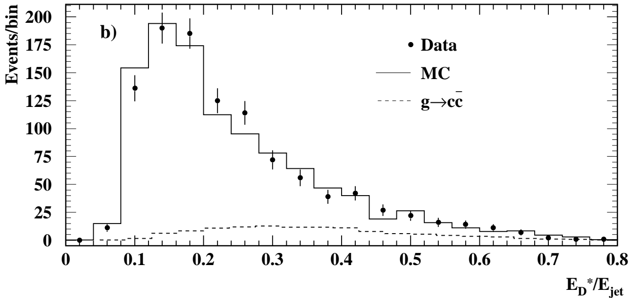
Figure 4: (a) The distribution of the difference of the invariant mass between the D^{*\pm} candidate and the D^0 candidate, \Delta M . The solid curve represents the estimated background shape. An estimated 137 \pm 13 D^{*\pm} candidates are above the background fit around 0.145 \text{ GeV}/c^2 . (b) Ratio of the D^{*\pm} candidate energy to the jet energy for candidates in the selected gluon jet after applying the combinatorial rejection criteria. The solid line shows the Monte Carlo spectrum with the g \rightarrow c\bar{c} component scaled to measured value in the D^{*\pm} analysis ( g_{c\bar{c}}=0.04 ), and the dashed histogram shows the spectrum for true D^{*\pm} mesons from g \rightarrow c\bar{c} scaled to the measurement area.
