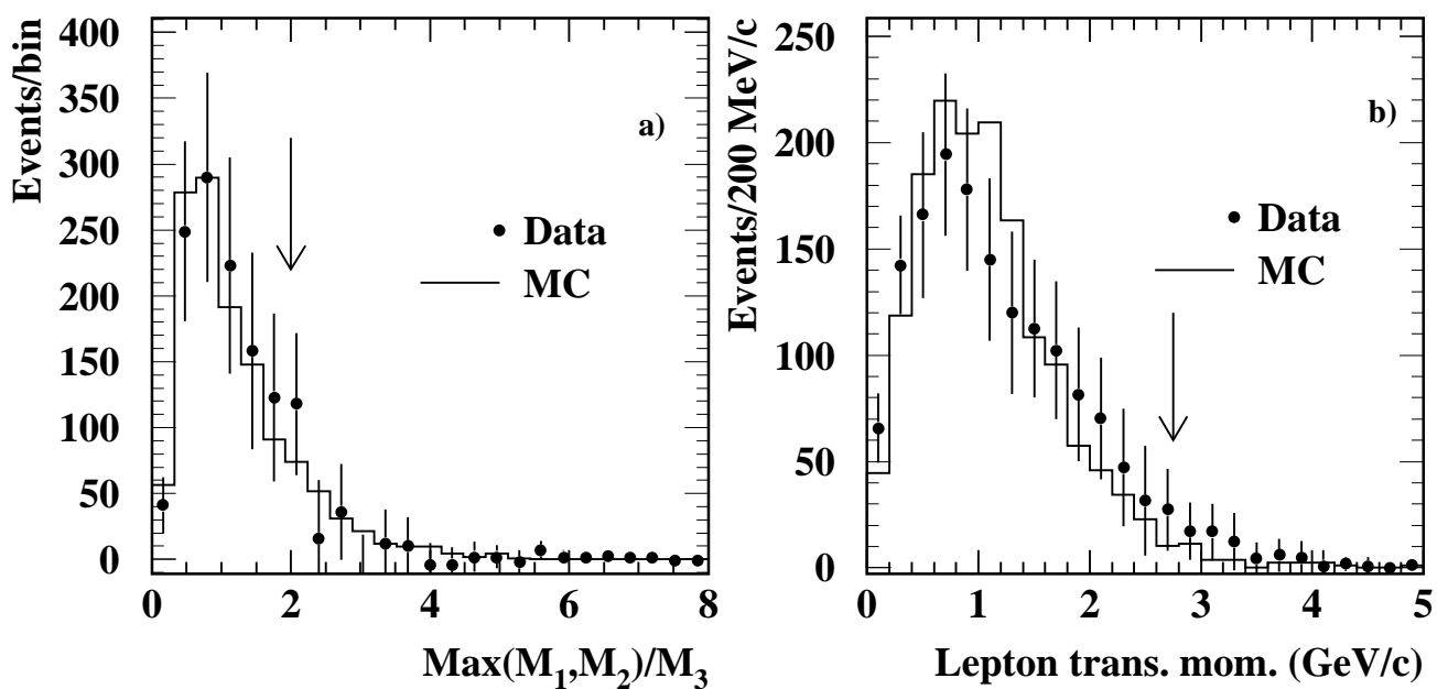
Figure 3: Distributions of a) \text{Max}(M_1, M_2)/M_3 , b) lepton transverse momentum for background subtracted data (points) and for g \rightarrow c\bar{c} Monte Carlo scaled to the average lepton analysis g_{c\bar{c}} result (solid line): All the selection criteria described in the text were applied with the exception of the variable in each plot where the cut is shown by the arrow. The error bars shown represent the statistical and systematical uncertainties combined.
