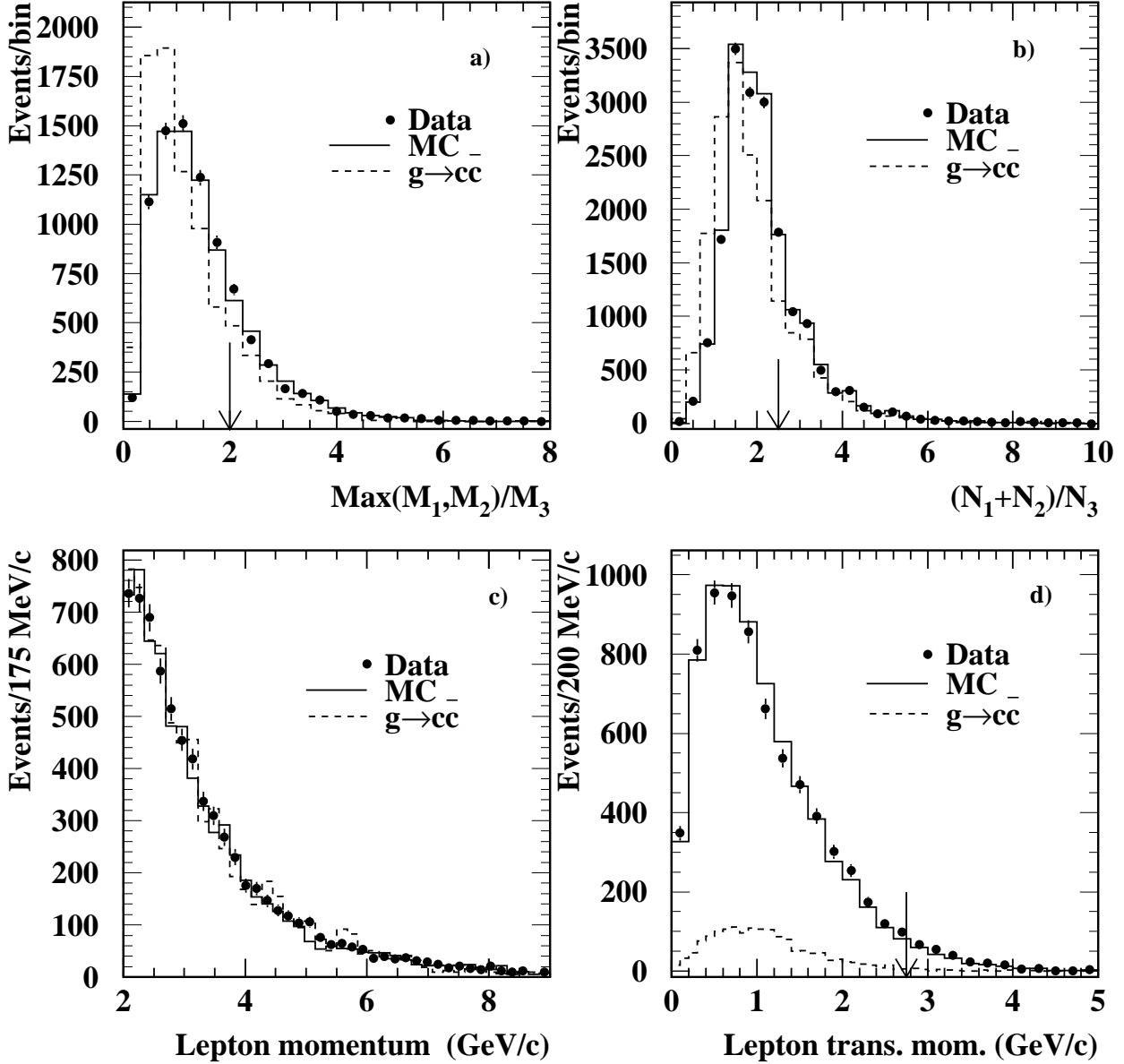
Figure 2: Comparison of data and Monte Carlo for the lepton analysis (histograms represent the Monte Carlo and data are represented by the points, the dashed histograms show the g \rightarrow c\bar{c} spectrum). Monte Carlo distributions (solid and dashed histograms) are normalised to the number of hadronic events in the data. a) Ratio of the maximum mass of the first two jets with respect to the third jet for events that passed the lepton selection and the b-tagging neural network rejection; b) ratio of the multiplicity of tracks and unassociated clusters in the first two jets with respect to the third jet for the events in a); c) lepton candidate spectrum for events passing all the selection criteria; d) lepton candidate transverse momentum spectrum for events passing all but the transverse momentum criteria with the g \rightarrow c\bar{c} spectrum scaled to the signal area. The arrows in a), b) and d) show the cut value used in this analysis. Events below these values were accepted.
