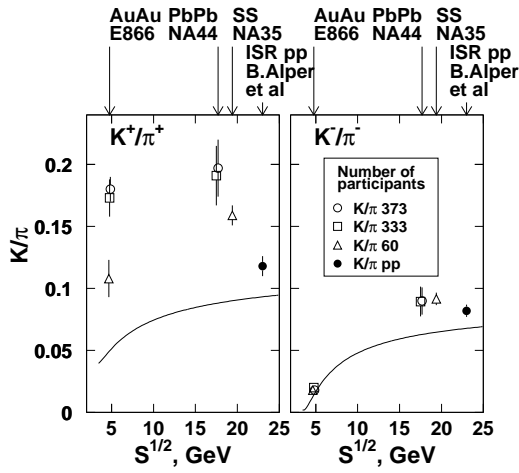
Fig. 3. K/\pi ratios in symmetric systems at midrapidity |y - y_{CM}| \leq |y_{proj} - y_{targ}|/8 . The solid line shows full solid angle K/\pi in p+p collisions from the interpolation [19]. The data points from other experiments result from an interpolation in y to the midrapidity interval. The E866 data points [17] are also interpolated in the number of participants, for comparison with the SPS data.
